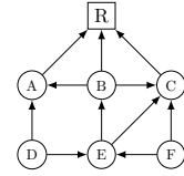
Figure 1: A DODAG.
