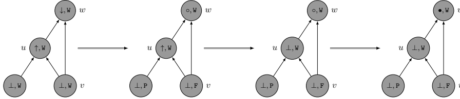
Figure 5: Cleaning children before sending up the token in a triangle: \text{play}_v = F .
