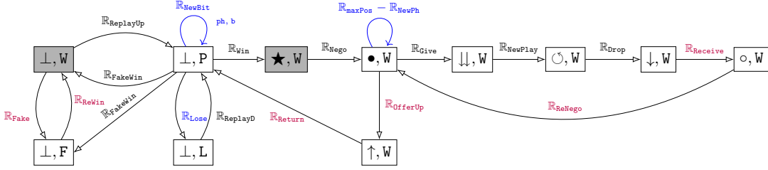
Figure 6: Chain of the states taken by a node during the execution of the algorithm. The update of c_v is represented by color gray. Rules in blue corresponds to the negotiation. Rules in red correspond to the sending of a token from a child to a parent. Rules in black correspond to the sending of a token from a parent to a child.
