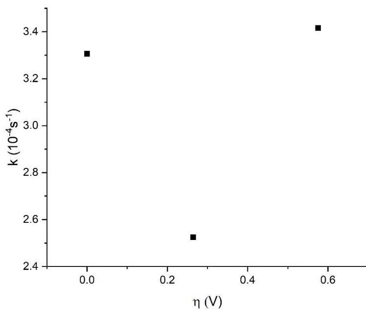
Figure S5: Kinetic constant k (surface path) as a function of applied overvoltage obtained for a second LNO symmetrical cell during POIE at P_{\text{O}_2} = 50 mbar at 700^\circ\text{C} .
