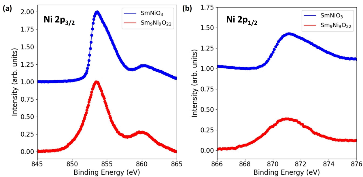
Figure S13: HAXPES comparison of Sm 9 Ni 9 O 22 and SmNiO 3 for (a) Ni 2p 3/2 and (b) Ni 2p 1/2 core levels. The measurements were done in a bulk sensitive mode, probing the whole thin-film. In both, Sm 9 Ni 9 O 22 has a low binding energy (LBE) shoulder, indicative of the Ni 1+ in the square-planar sites. The bulk-probing capacity of HAXPES makes it insensitive to possible surface contaminations or artefacts. One noticeable difference is the presence of a low binding energy (LBE) shoulder for Sm 9 Ni 9 O 22 compared to SmNiO 3 that can also be attributed to the Ni 2+ and Ni 1+ sites.
