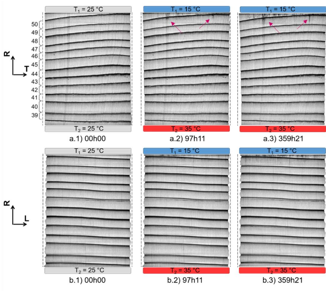
Figure 7: Tomographic sections through the axis of the sample during phase 1 a) in the R-T plane and b) in the R-L plane. The dark grey level is equivalent to the denser material than the light grey level
