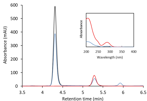
Figure 4: Enlargement of the chromatogram traces of the reaction mixture in presence (blue) and absence (black) of HRP and of the synthetic dimer (red) ( \lambda_{\text{abs}} = 220 nm). The full chromatogram traces are shown in Figure S7. Inset: UV spectra of the synthetic dimer (red) and the enzymatic product (blue) at a retention time of 5.3 min (TRIS/HCl, 10 \text{mmol}\cdot\text{L}^{-1} , pH 7.0, [MHPA] = 1 \text{mmol}\cdot\text{L}^{-1} , [HRP] = 0 or 10^{-10} \text{mol}\cdot\text{L}^{-1} and [ \text{H}_2\text{O}_2 ] = 0.5 \text{mmol}\cdot\text{L}^{-1} ).
