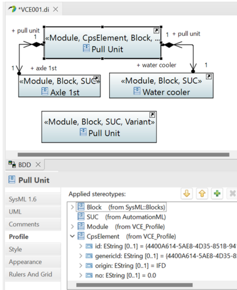
Fig. 6. Excerpt of an annotated SysML model of the DS.
