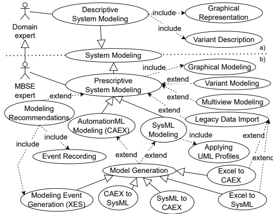
Fig. 3. Actors and use cases of our field of investigation.
