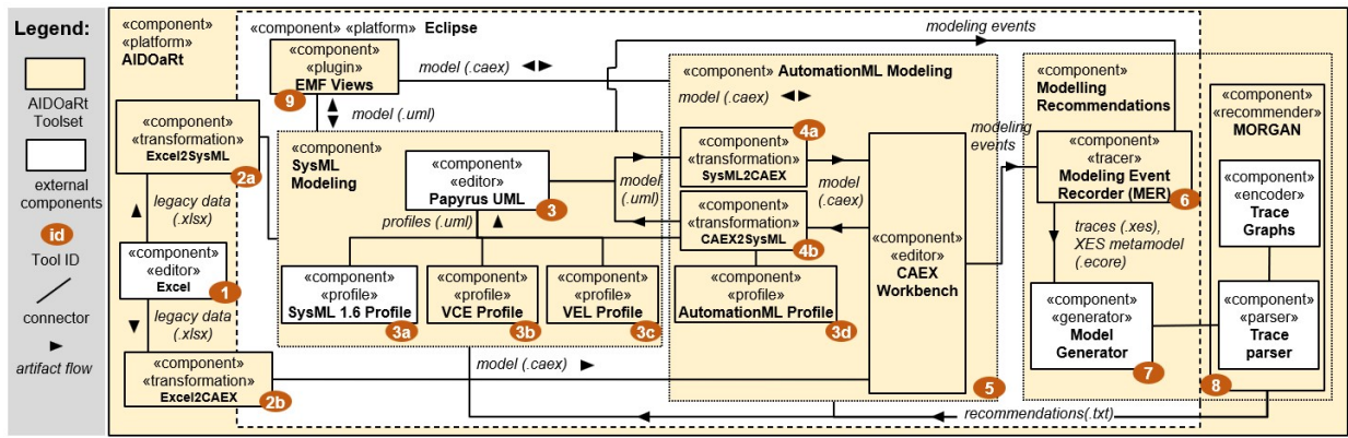
Fig. 4. The solution architecture for VCE challenges as part of the larger AIDOaRt framework.
