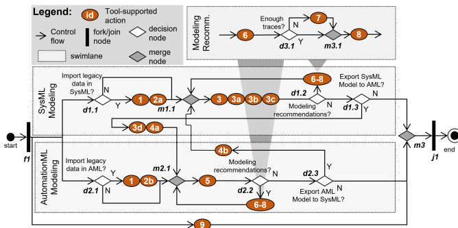
Fig. 5. The engineering workflow enabled by the solution architecture.
