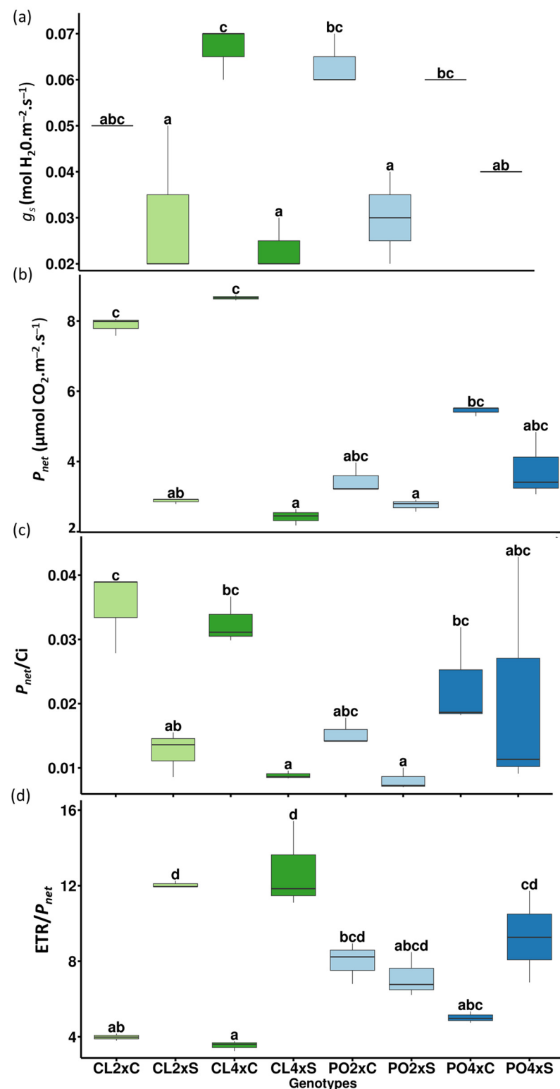
Figure 6. Photosynthetic performances under control (C) and salt stress conditions (S). Stomatal conductance ( g_s ) (a), net photosynthesis ( P_{net} ) (b), carboxylation efficiency ( P_{net}/c_i ) (c) and indicator of electron transport utilized by acceptors other than CO 2 ( ETR/P_{net} ) (d). Data represent 3 independent measurements ( n = 3 ) after four weeks of salt treatment (90 mM). Significance of the values were analyzed using Kruskal–Wallis test ( p > 0.05 ) and mean comparison using Dunn’s test. C and S represent Control and stressed plants, respectively. Groups are separated by letters. Each group is assigned one or more letters. Groups sharing the same letter are not significantly different. Letter displays a clear and succinct way to present results of multiple comparisons.
