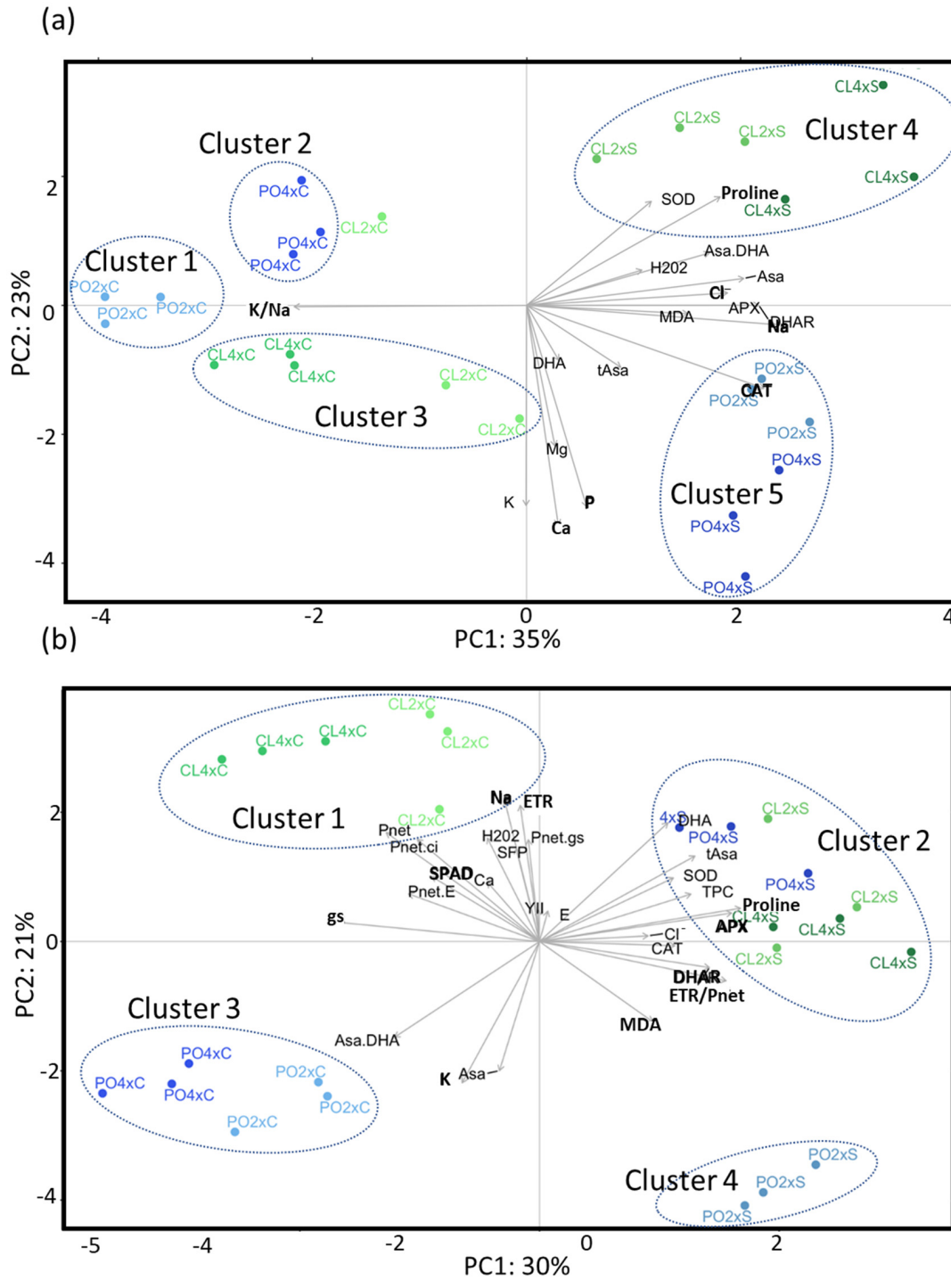
Figure 2. Discriminant analysis of biochemical and photosynthetic variables under control (C) and stress conditions (S). PLS-DA biplot represents discrimination of Cleopatra (CL) and trifoliolate orange (PO) genotypes at two ploidy levels (2x, 4x), with (S) and without salt stress (C), in roots (a) and leaves (b). Measurements were performed at W4 (90 mM). Colored dots represent biological replicates for each genotype. sPLS-DA selected variables were represented in bold.
