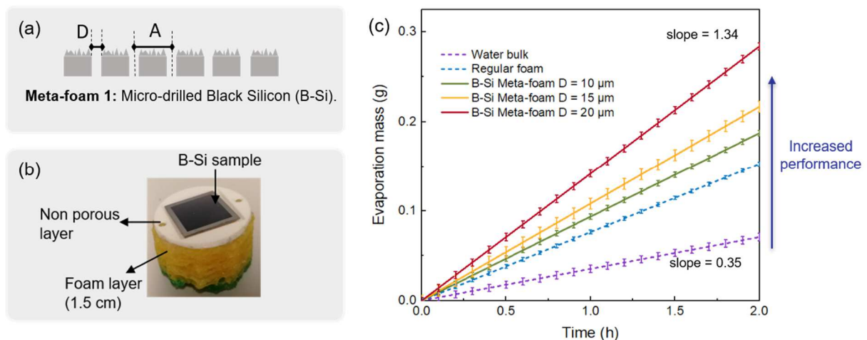
Figure 3. 2D black silicon meta-foams: (a) schematic cross-sectional description, (b) photo of the assembly used for the experiments (c) measured evaporation rates (water loss) on the three different meta-foams, compared with the evaporation rate of bulk water and evaporation rate using a regular foam.
