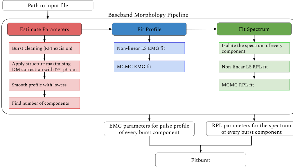
Figure 1. Flowchart showing the Baseband Morphology Pipeline. Path on the left involves extracting the Stokes Intensity (I) data products from the beamformed file, dedispersing and cleaning the spectra, getting the burst profile and estimating the number of sub-bursts/peaks to fit for. The middle portion indicates the process of extracting initial guesses on the temporal profile of each sub-burst, first by a Least Square (LS) fit and then by MCMC sampling using an Exponential Modified Gaussian (EMG). As indicated in the right hand column we then estimate the spectral parameters using the same methods assuming a Running Power Law (RPL) model. The resulting datafile along with initial guesses are then provided to fitburst .
