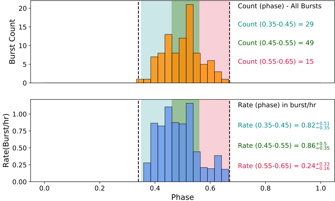
Figure 5. Burst count and rate variation with phase. We folded our burst arrival times at a period of 16.34 days with reference MJD 58369.40. We did the same with our calculated exposure and estimated the burst rate of FRB 20180916B in different phase bins. The top panel shows the burst count distribution of all the bursts detected by CHIME/FRB till 2021 December 31. We detect most of the bursts near the peak activity phase of CHIME/FRB i.e., 0.45-0.55. The bottom panel shows the rate. Here we have excised the bursts detected during days of low sensitivity and those detected outside the FWHM at 600 MHz to get true estimate on the rate. The rate is maximum in the phase range 0.45-0.55 (green). We also show the rates in phases earlier i.e 0.35-0.45 (blue) and later, i.e., 0.55-0.65 (red). The three rates are consistent within error bars (95%) assuming a Poissonian process. See Section 3.4 for details.
