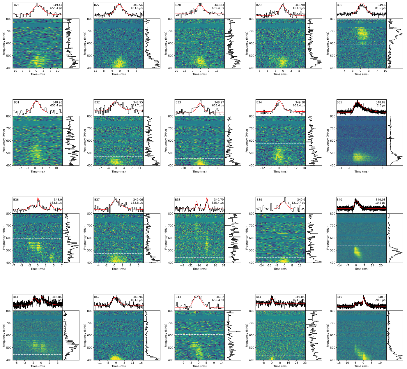
Figure 9. Continued from Figure 8
