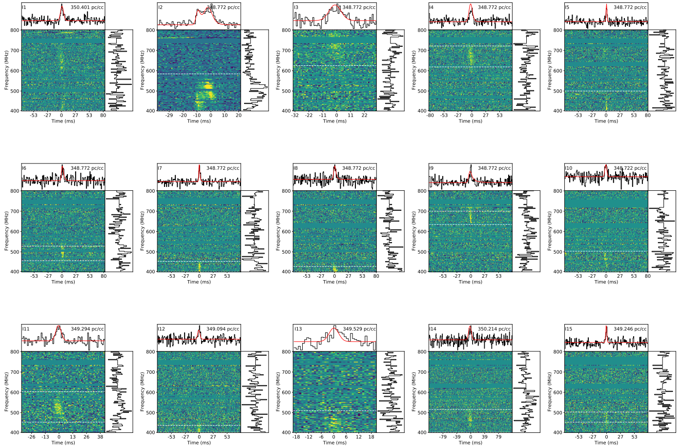
Figure 10. Waterfall figure similar to Figure 8 showing bursts detected from FRB 20180916B only with Intensity data from 20th September 2020 till 31st December 2021. All of these bursts are shown at a resolution of 0.983 ms and 128 channels
