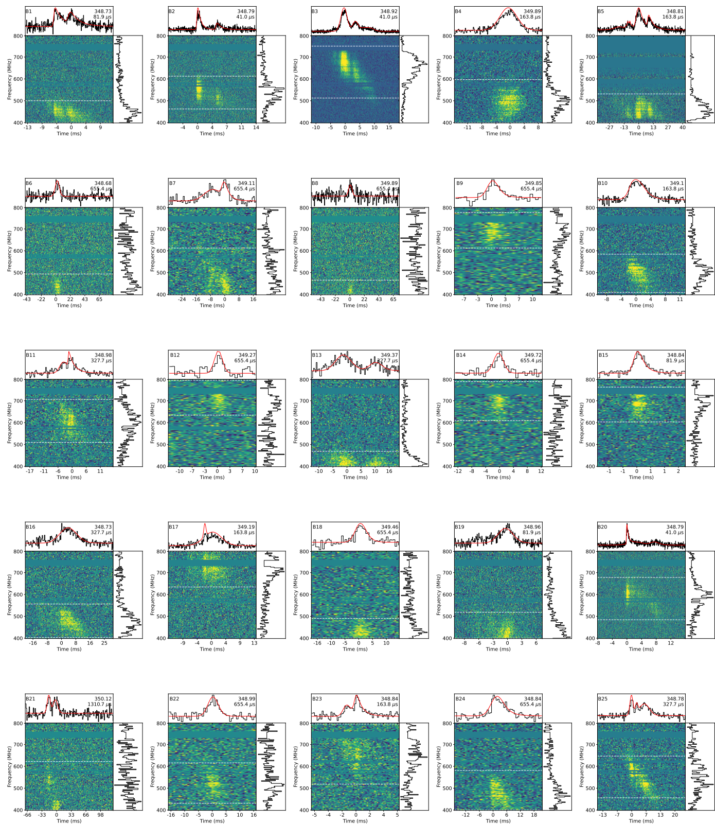
Figure 8. Figure showing bursts detected by the baseband system from FRB 20180916B dedispersed at their structure maximizing DM. In each sub-figure the top panel shows the time-series with red line showing the best fit, the panel below it shows the dynamic spectra and finally to the right of it is the frequency distribution of the power. The white-dotted lines show the extent of bandwidth. In top right we see the DM it has been dedispersed to and the time-resolutions its been plotted in microseconds, the top left shows the burst number. The number of channels here is 128.
