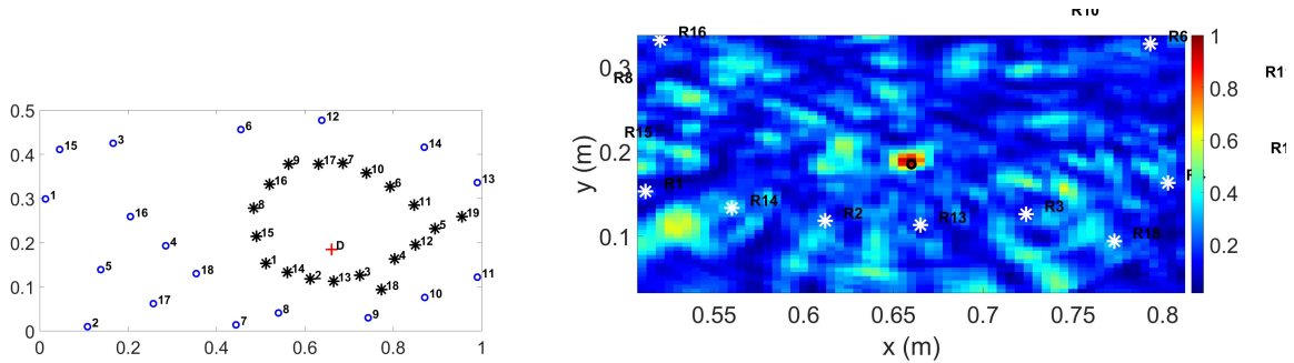
Figure 6. (Left) Schematic configuration of the considered experiment. (Right) Passive image of a CAN obtained with N_s = 18 and N_r = 19 , located at (0.66, 0.185) m. The circles denote noise emitters, the asterisks are for receivers and the cross represents defect position.
