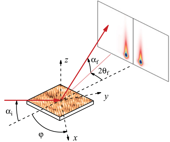
FIG. 1. (Color online) Schematic drawing of the scattering geometry used to perform 3D GISAXS reciprocal space mapping. \alpha_i denotes the angle of incidence, \varphi is the in-plane rotation angle, and (2\theta_f, \alpha_f) are the in-plane and out-of-plane angles of emergence. The z direction is normal to the sample surface, while the x and y directions are in the surface plane.
