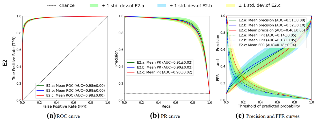
Fig. 15 Over-representing the negative class \neg C reduces false positives—on CAMELYON16. Mean curves with standard deviation (std. dev.) of experiments E2.a (for balanced distribution), E2.b (for over-
