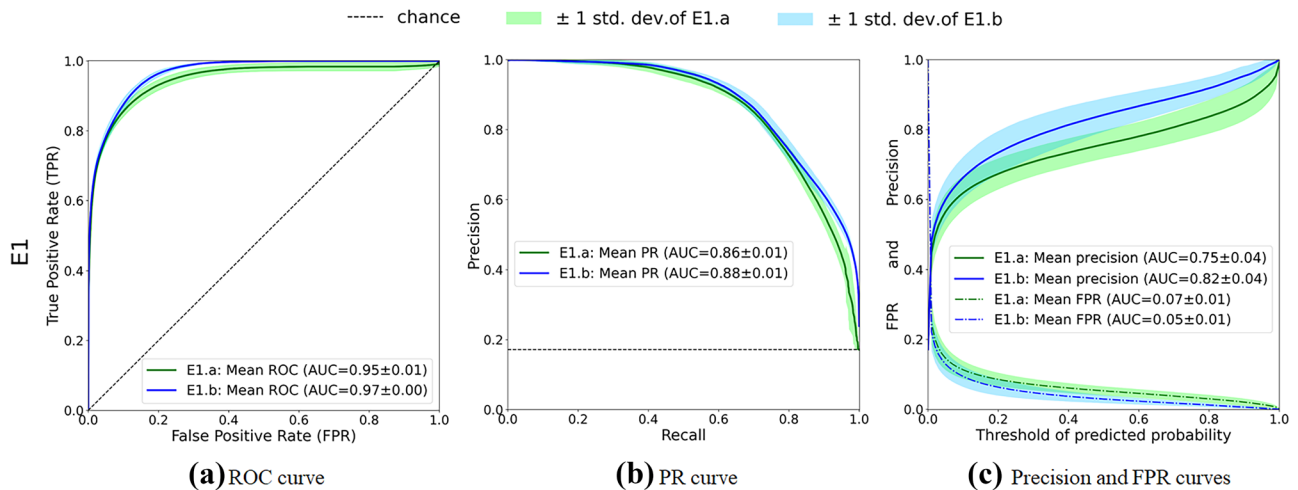
Fig. 7 Natural distribution (E1.b) is better than balanced distribution (E1.a) ( \neg H1 ). Mean curves for (a) the ROC curve, (b) the PR curve, and (c) the precision and FPR curves. Sub-figures are obtained for 10 runs for balanced distribution (E1.a, lines in green) and for natural
