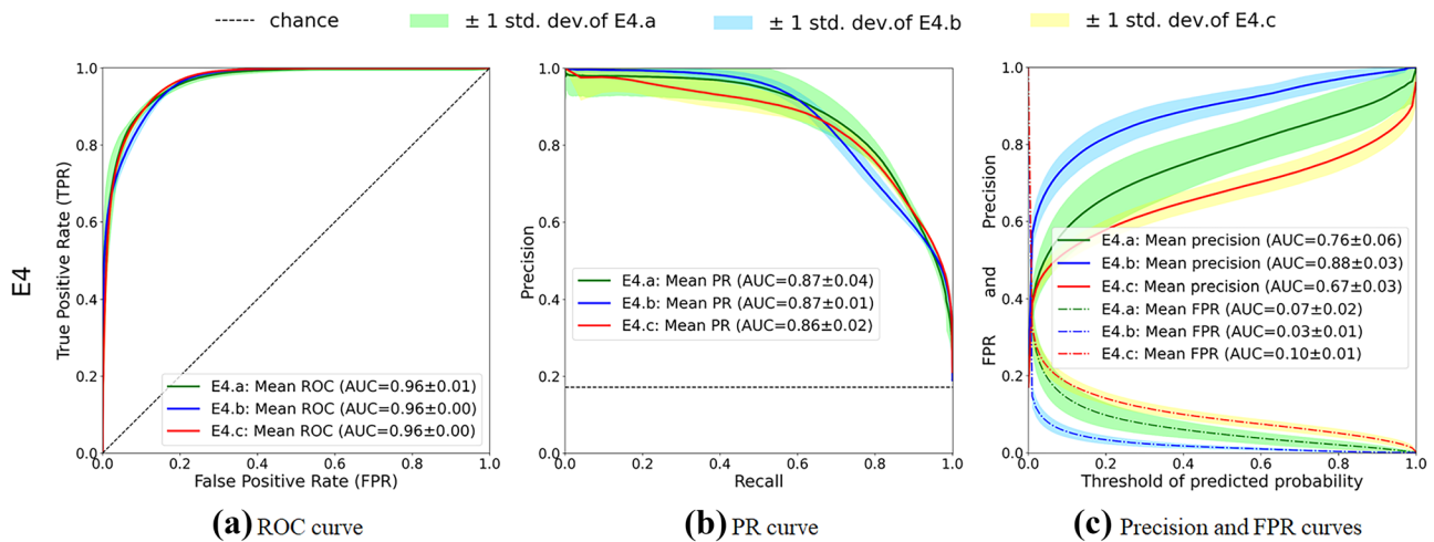
Fig. 13 Non-ROI data are useful (H4 hypothesis). Mean curves with standard deviation using E4 settings (Table 5) where \odot examples replace some C examples and some \neg C examples: E4.a (for balanced
