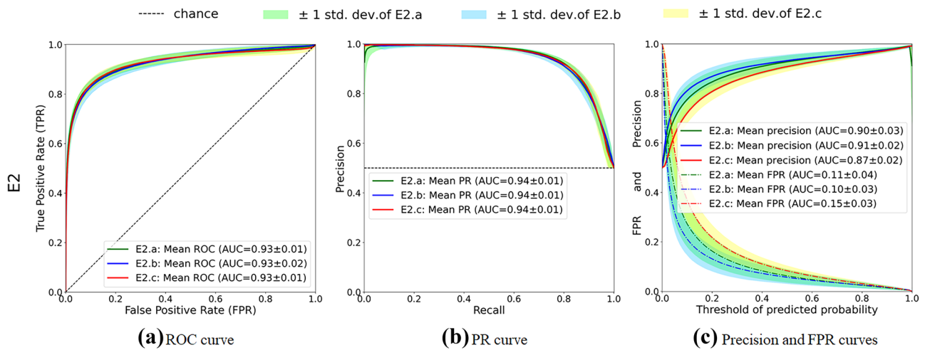
Fig. 14 Over-representing the negative class \neg C reduces false positives—on PCam. Mean curves with standard deviation (std. dev.) of experiments for balanced distribution (E2.a), for over-represented \neg C (E2.b), and for over-represented C (E2.c) on PCam
