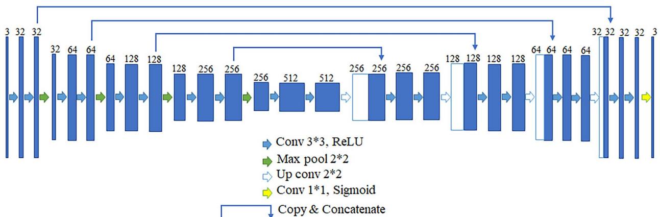
Fig. 6 The U-net architecture: the first and last layers represent the input and the output of the model respectively, while the layers that come after an arrow indicate the output of the operation denoted by
