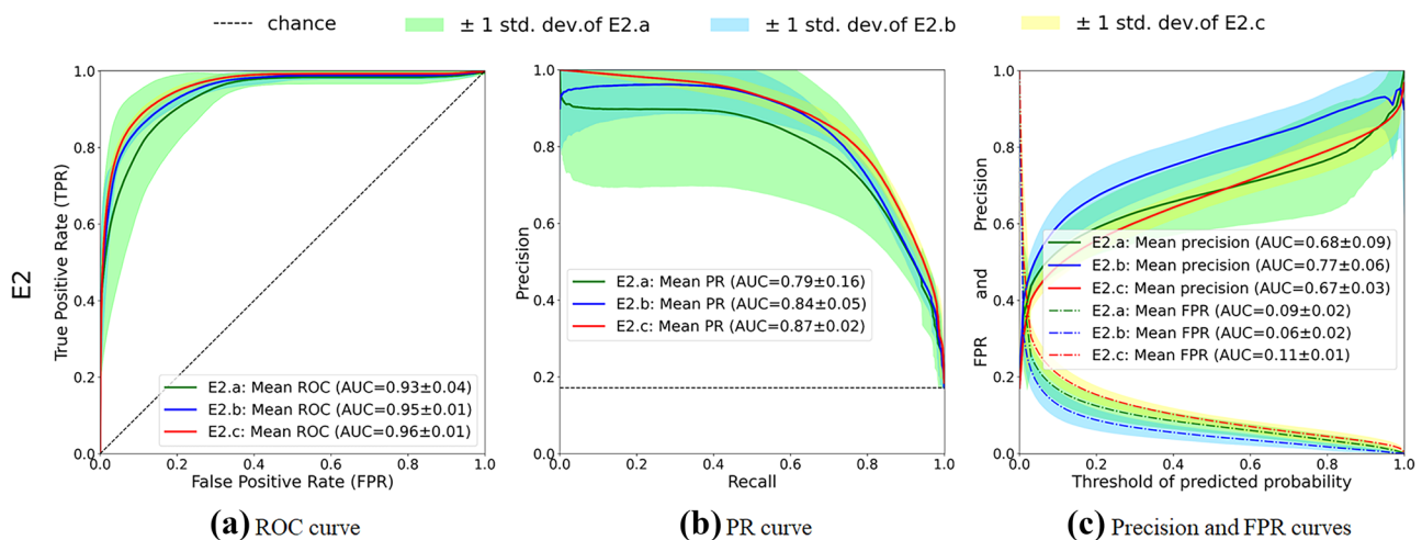
Fig. 9 Over-representation of negative classes \neg C reduces false positives (hypothesis H2). Mean curves with standard deviation for experiment settings E2.a (for balanced distribution in the training set, green),
