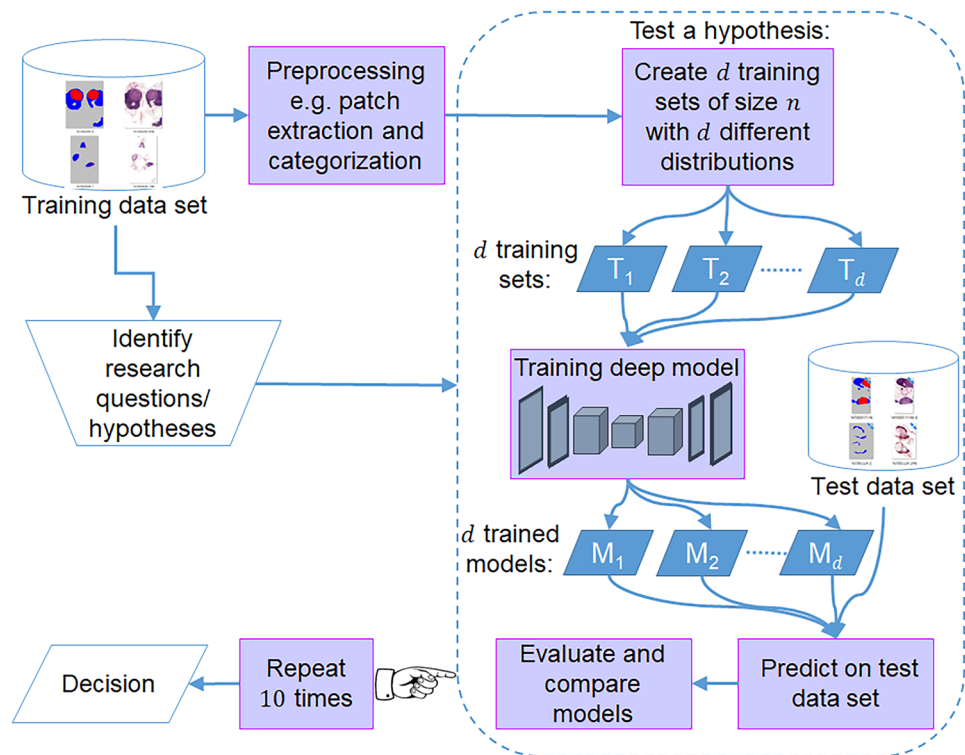
Fig. 1 Our methodological framework. To answer the general question of what the optimal class distribution of the training set should be, we created d training sets with n patches and d different distributions. We then trained d models corresponding to each distribution that we tested on the same unseen test set. The training data distribution of the best model for test data was considered as the best distribution. We repeated each experiment 10 times and calculated the mean to be able to make the final decision
