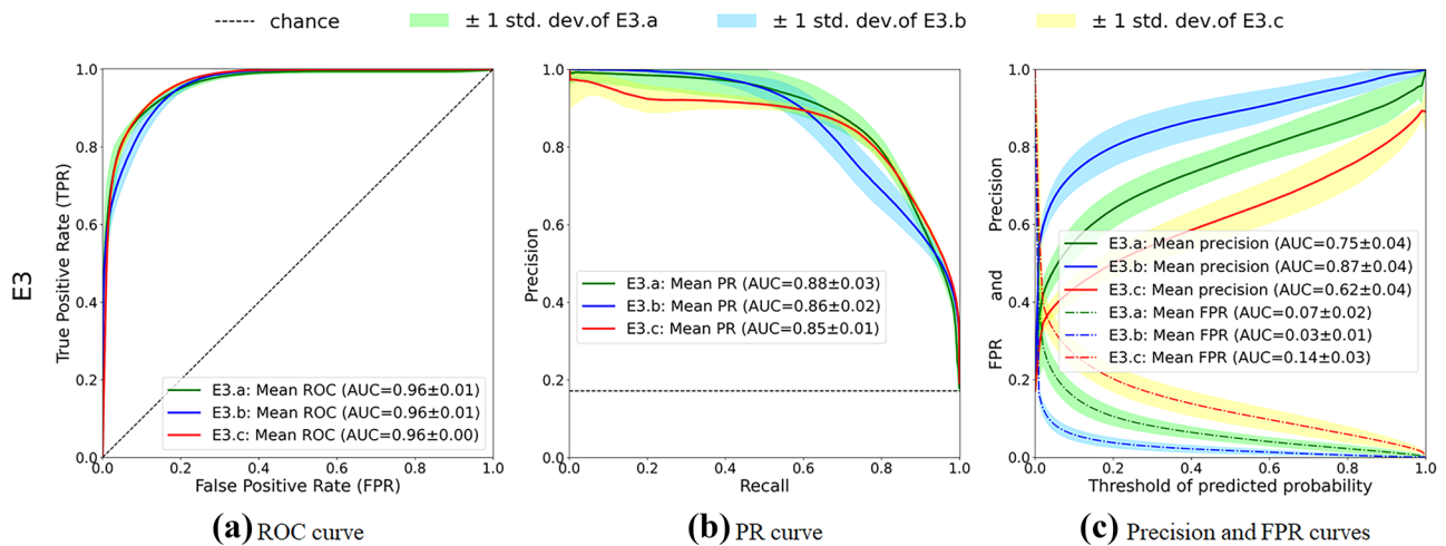
Fig. 12 Multi-label examples give extra advantages over single-label examples (H3 hypothesis). Mean curves with standard deviation using E3 settings (Table 4) where there are multi-label examples:
