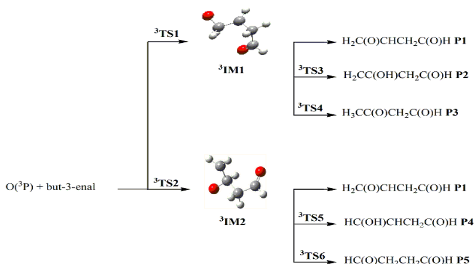
Scheme 1. Schematic representation of the different O-addition paths of the studied reaction of but-3-enal with O( 3 P).
