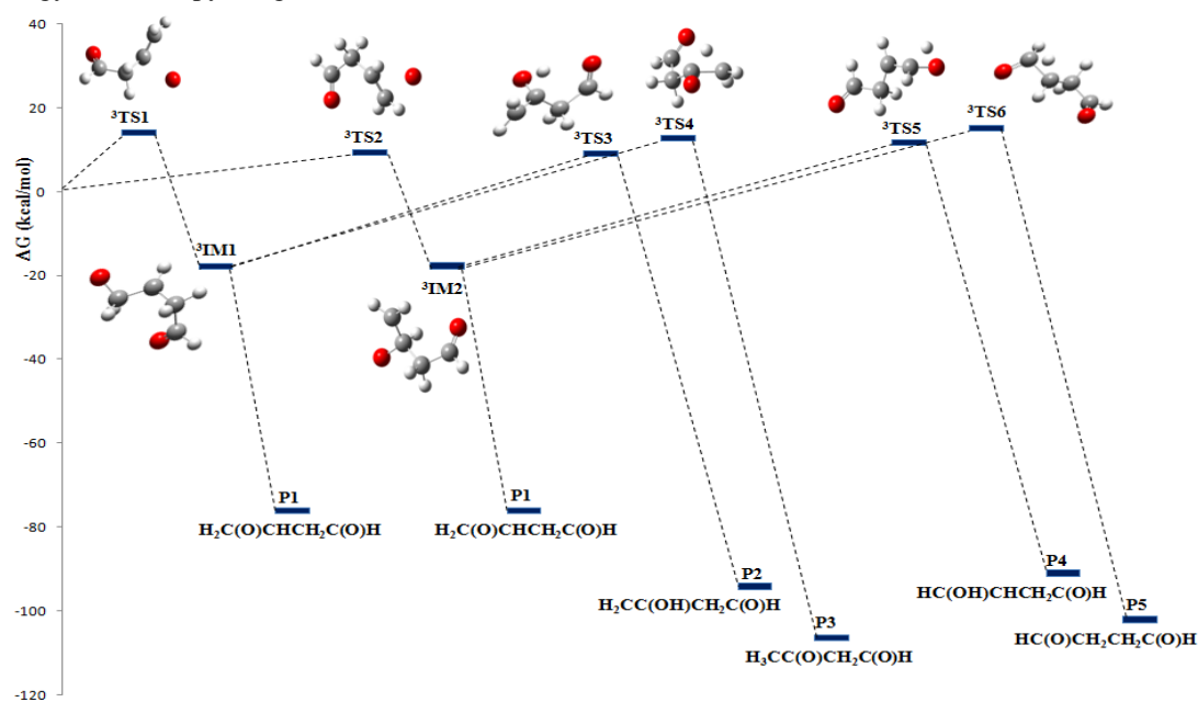
Figure 1. Energetic profile in kcal/mol of the different channels for the reaction pathways addition of but-3-enal with O( 3 P) which is calculated at G3 level at 298.15 K.
