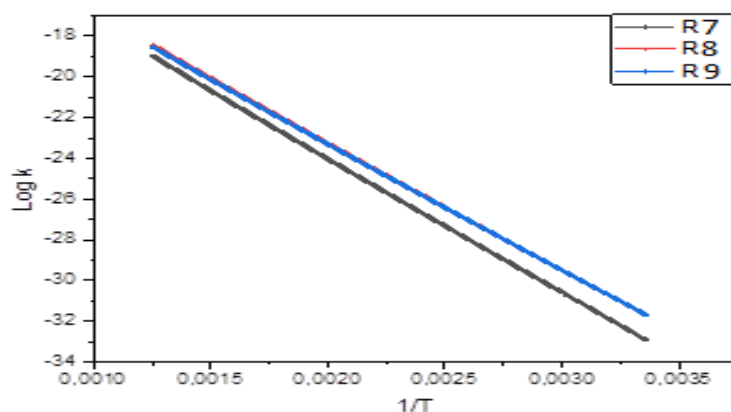
Figure 4. Arrhenius plots for the H-abstraction reaction of but-3-enal with O( 3 P) in the range of 298-798 K calculated at the MP2 level of theory.
