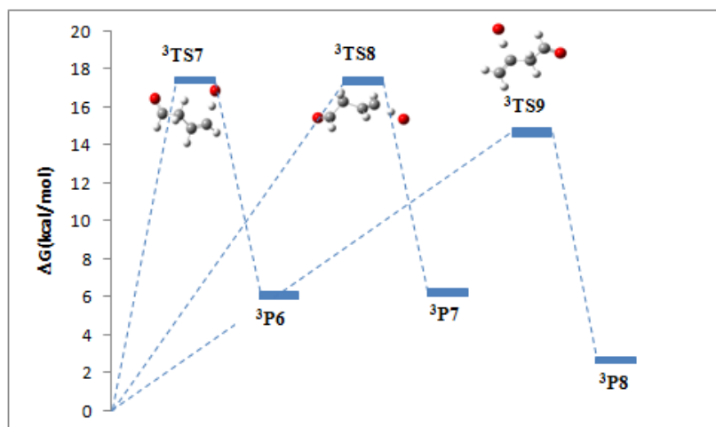
Figure 2. Energetic profile in kcal/mol of the three possible H-abstraction channels of but-3-enal with O(^3P) at G3 level at 298.15 K.
