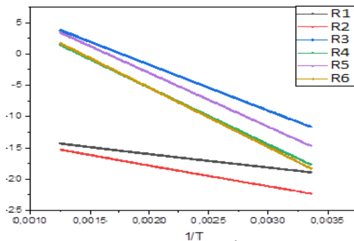
Figure 3. Arrhenius plots for the addition reaction of O(^3P) to but-3-enal in the range of 298-798K calculated at the MP2 level of theory.
