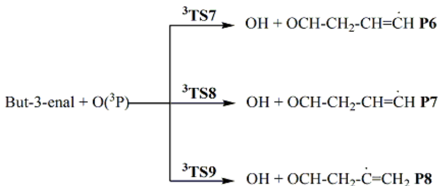
Scheme 2. Schematic representation of the three possible H-abstraction channels of but-3-enal by oxygen atom.
