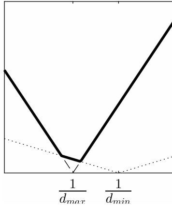
Fig. 2. This plot displays values of c_2 on the x-axis. The dotted line corresponds to the function |d_{\min}c_2 - 1| , the dashed line plots the function |d_{\max}c_2 - 1| and the solid line depicts the bound which is to be minimised in (8), i.e., \max(|d_{\max}c_2 - 1|, |d_{\min}c_2 - 1|) .
