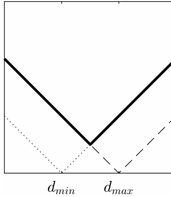
Fig. 1. This plot displays values of b_1 on the x-axis. The dotted line corresponds to the function |d_{\min} - b_1| , the dashed line plots the function |d_{\max} - b_1| and the solid line depicts the bound which is to be minimised in (4), i.e., \max(|d_{\max} - b_1|, |d_{\min} - b_1|) .
