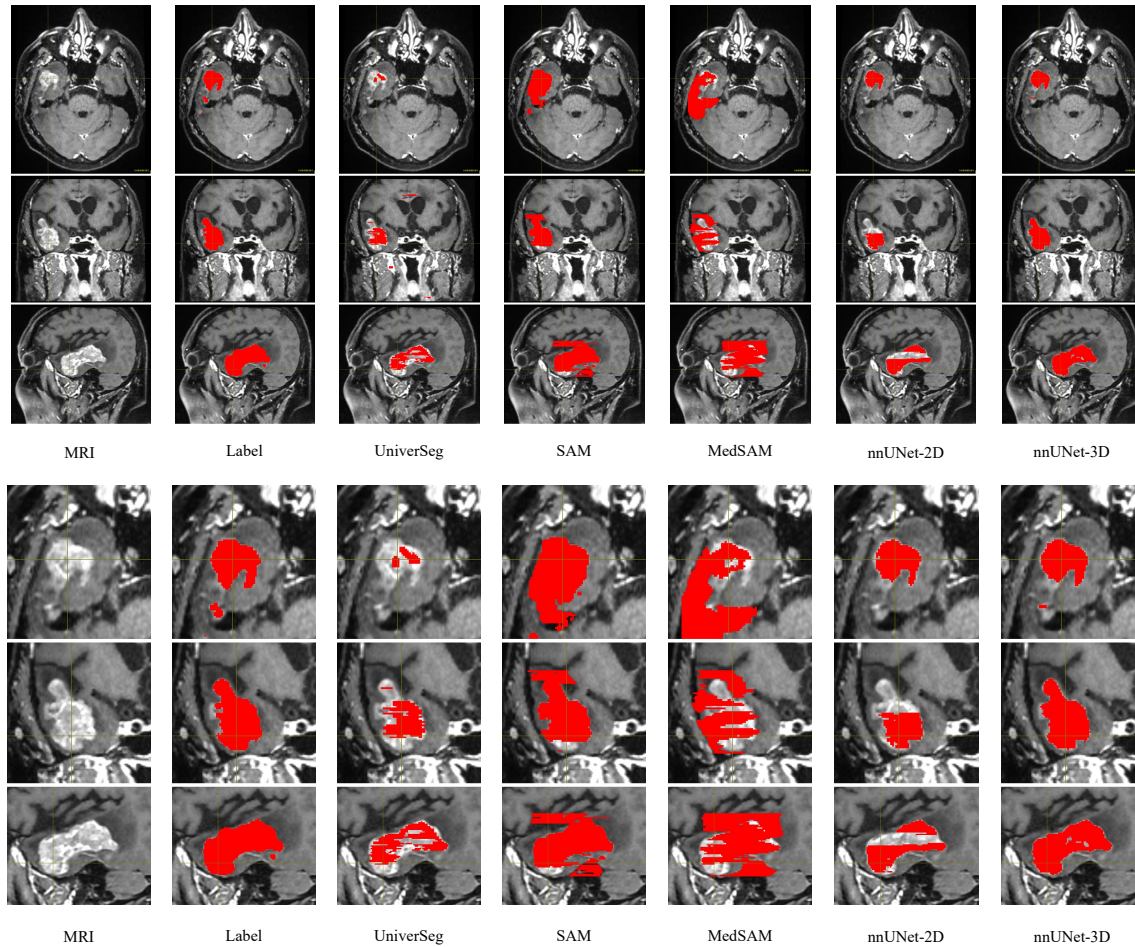
Figure S6: Ground-truth label vs predictions on lymphoma data: case (a). Upper row: full MRI. Lower row: zoom-in. FMs results are all very poor. They are all inconsistent across slices. UniverSeg vastly underestimates the lesion boundaries but also produces many produces false positives remote from the lesion (these can be better appreciated in the 3D renderings in Figure 3). SAM and MedSAM both provide massive over- and under-estimations depending on the area. nnUNet-2D completely misses some slices as was already clear from Figure 3. The result of nnUNet-3D is in general acceptable even though it misses small parts of the tumor. Note that we can also see that the ground-truth label has some minor imperfections.
