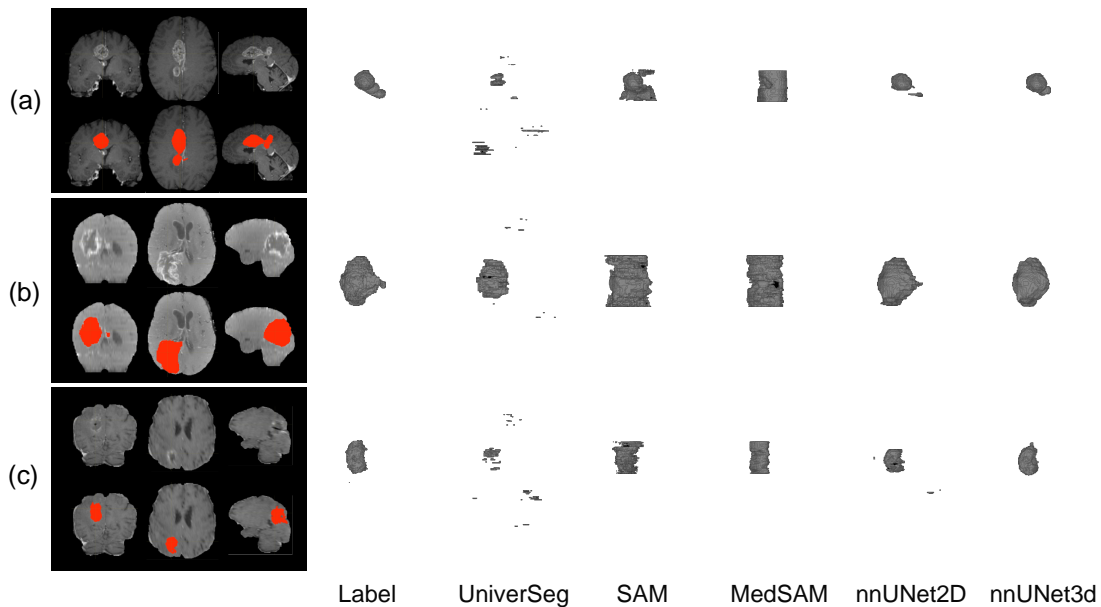
Figure S9: Ground-truth label vs predictions on three representative patients from MSD-BraTS. Left: ground-truth superimposed on MRI. Right: 3D renderings of ground-truth (label) and of predictions with different methods. As for lymphomas, FMs do not recover the 3D shape of the tumor. Besides, UniverSeg produces a lot of false positives distant from the lesion.
