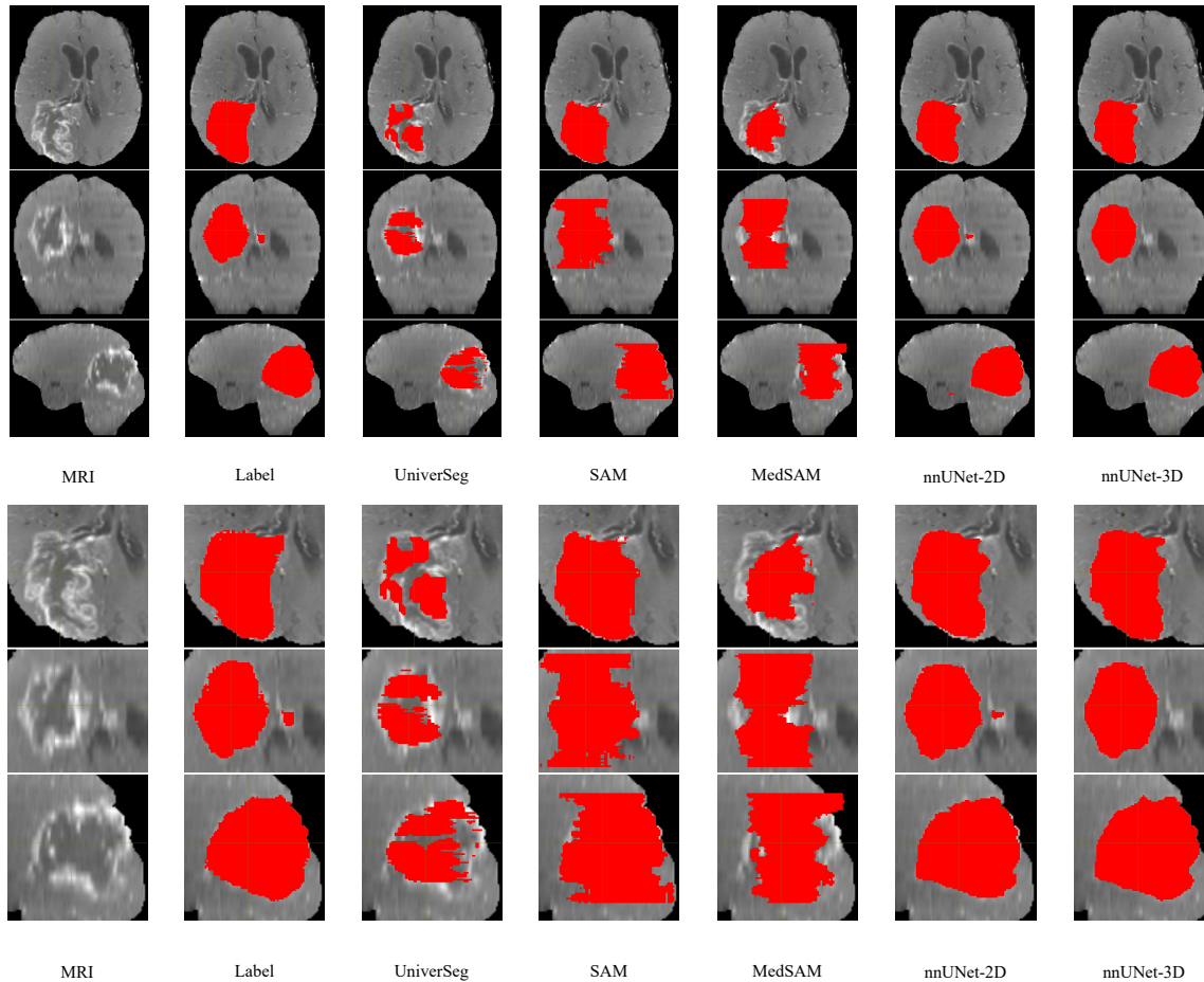
Figure S11: Ground-truth label vs predictions on MSD-BraTs data: case (b). Upper row: full brain. Lower row: zoom-in. All FMs result in a poor segmentation. UniverSeg mostly undersegments the tumor. SAM and MedSAM struggle finding the contours, alternating between over- and under-segmentations. nnU-Net-2D and nnU-Net-3D both do a decent job even though the 3D version misses a part of the tumor which is partly recovered by the 2D model. The latter phenomenon was rarely found (in general, the nnU-Net-3D provides better results).
