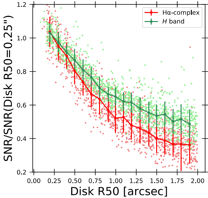
Fig. 14. S/N of the extracted H\alpha -complex measurements (red) and extracted continuum measurements (green) normalised by the median S/N for sources with a disk half-light radius ( R_{50} ) of 0''.25 as a function of the disk R_{50} . The lines and error bars show the normalised median S/N and MAD values calculated in disk R_{50} bins including a fixed number of 50 sources. Results are presented for a sub-sample of 1248 sources with all morphological parameters set at their default value (see Sect. 2.3.2) except the disk R_{50} , which varies from 0''.1 to 2'' .
