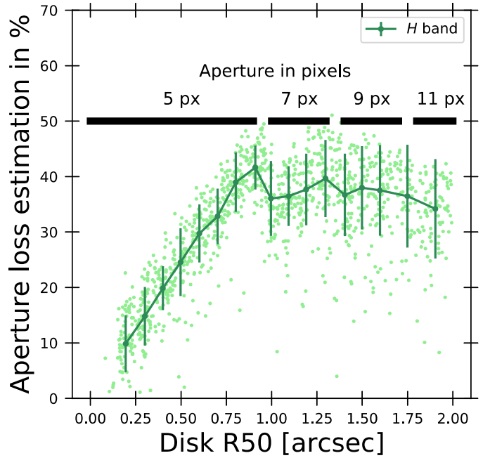
Fig. 15. Estimation of the aperture loss as a function of the disk R_{50} in arcseconds. The line and error bars are obtained calculated the median aperture loss obtained on disk R_{50} bins including a fixed number of 50 sources. The method to estimated the loss due to the aperture is described in the text. The results are presented for a sub-sample of 1248 sources with all morphological parameters set at their default value (see Sect. 2.3.2) except the disk R_{50} , which varies from 0''.1 up to 2'' . We indicated with black thick lines the range of sizes corresponding to the different apertures in pixels, recalling that the spatial resolution of the NISP instrument is 0''.3 .
