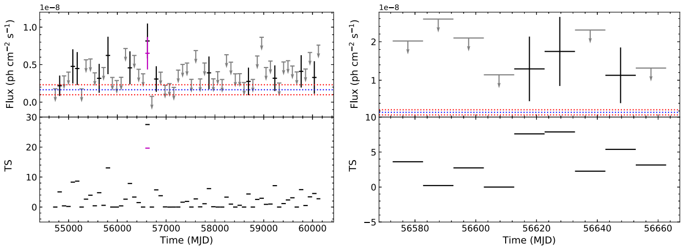
Figure 4. Long-term light curve and TS evolution for M5 in the energy range of 0.1–500 GeV. Left: 90-day binned light curve. Right: a zoom-in around bin 21 of the 90-day light curve with a binning of 10 days (from MJD 56572 to MJD 56662). Flux upper limits at the 95% CL are shown as arrows for bins when the source had TS < 4 . Blue dotted line: average flux in the broad band. Red dotted lines: 1\sigma uncertainties on the average flux. The magenta marker indicates the flux and TS in bin 21 after taking into account the excess near M5.
