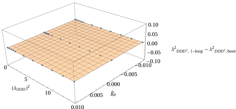
Figure 3. Difference between the perturbative prediction and the extrapolated bound on the (\lambda_{\text{DDD}})^2 OPE coefficient for varying c and \Delta_{\text{D}}, \Delta_{\text{D}^2} , following the perturbative prediction parametrized by \tilde{g}_\phi with \Delta_\phi = 1.5 . The yellow surface serves as a guide to the eye, excluding points above it.
