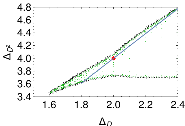
Figure 12. The combined \phi_{(3,3)} + \phi_{(1,3)} deformation of the (2, 1)_4 b.c. for \Delta_\psi = 3/2 . The solid line is the perturbative result of eq. (4.20), which appears to saturate the upper bound to the right of the (2, 1)_4 point, represented by the red circle.
