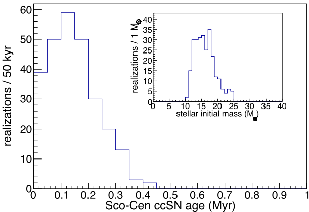
Figure 8. Age and stellar initial mass distributions for the Sco–Cen SN accelerating more than 50 per cent of the observed ^{60}\text{Fe} CR density measured by ACE/CRIS .
