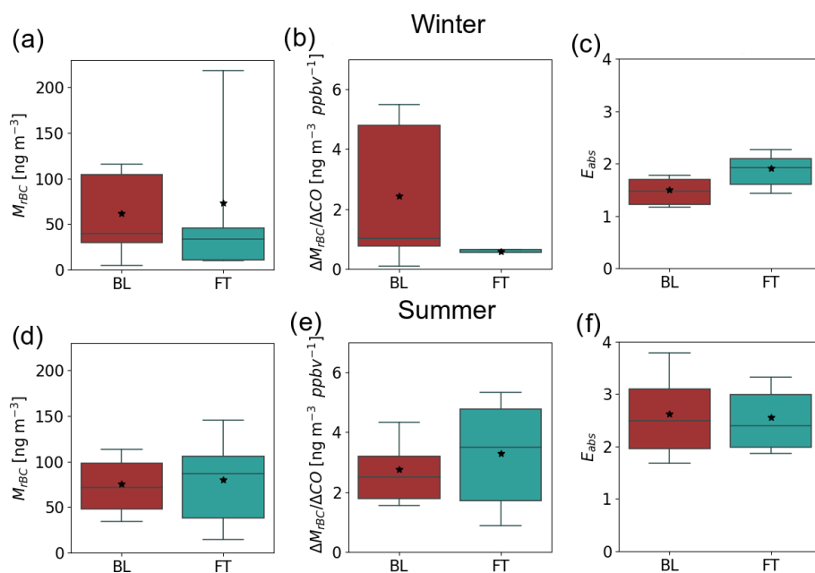
Figure 10. (a) rBC mass concentrations, (b) \Delta M_{\text{rBC}}/\Delta\text{CO} emission ratio and (c) E_{\text{abs}} as a function of the predominant influence at PDM in winter. The same for summer is given in (d), (e) and (f). Red boxplots represent PBL conditions, and green boxplots represent FT conditions. Precipitation events were filtered before analyses.
