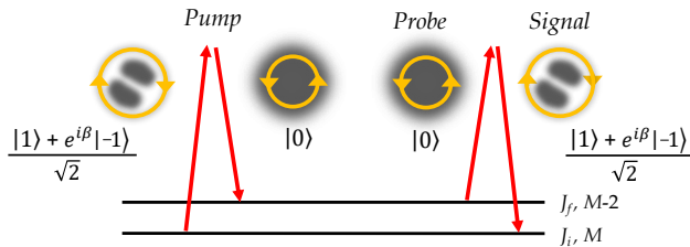
Figure 1 Coupling scheme for encoding structured fields embedding OAM modes into rotational states of molecules. The SAM conservation allows transitions \Delta J = J_f - J_i = 0, \pm 2 , \Delta M = +2 ( \Delta M = -2 ) for the probe (pump) interaction.
