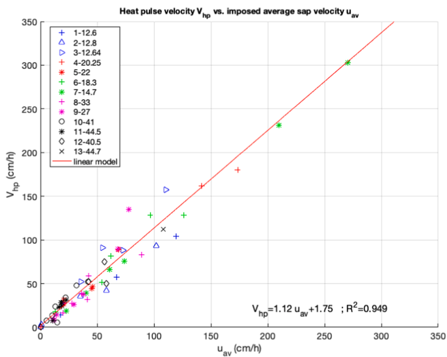
Fig. 5. Assessed heat pulse velocity V_{hp} versus average sap flow velocity u_{av} in the sapwood for the 13 stem samples. ( n = 82 ).
