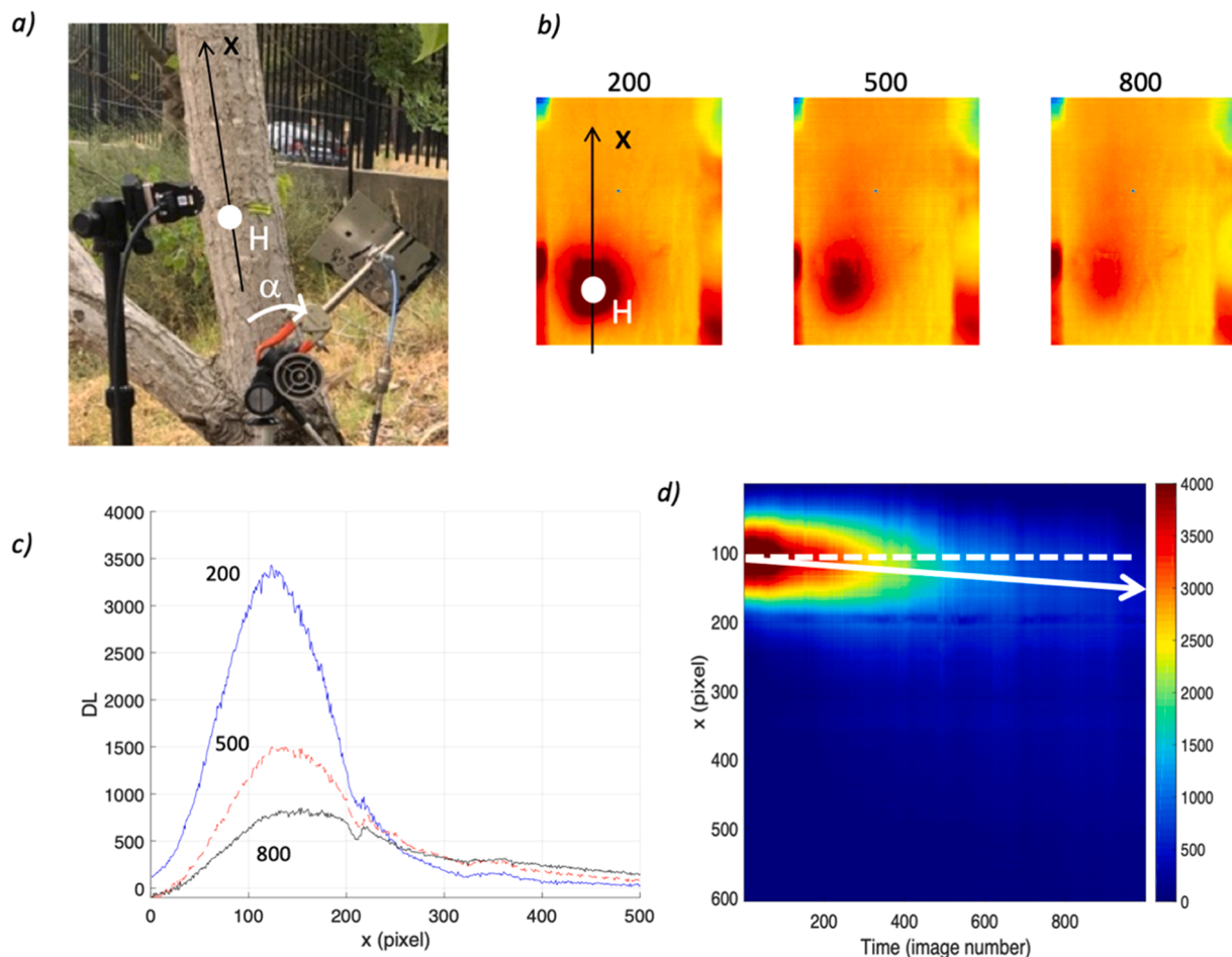
Fig. 7. Example of an outdoor test. (a) experimental setup on a poplar tree trunk (103 mm diameter) showing the microwave excitation point H (after a rotation \alpha of the antenna) and the infrared camera recording heat propagation in x direction. (b) Example of three thermal radiation images (number 200, 500, 800) showing the propagation and attenuation of the heat front. (c) thermal radiation profiles along x direction, at the same times. (d) spatiotemporal variations in the thermal radiation measured at the sample surface, showing the heat pulse propagation pattern (white arrow).
