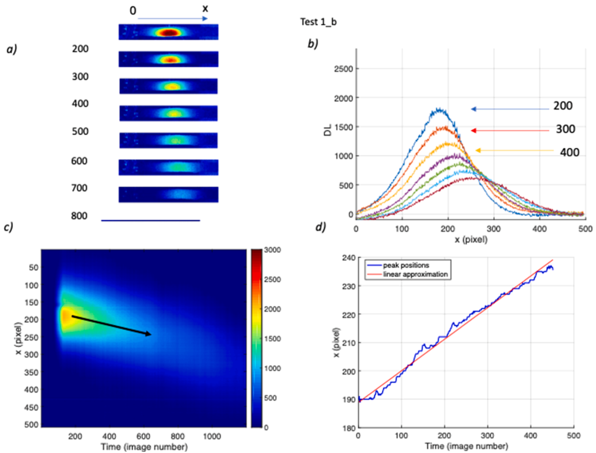
Fig. 3. Thermal images and heat pulse analyses for a small stem (sample 1, D_0=12.6 mm) and a mean flow velocity of 57.6 \text{ cm h}^{-1} (test 1_b; imposed flow of 0.0140 \text{ g s}^{-1} ). a) Example of seven thermal radiation images (number 200, 300,..., 800) showing the propagation and attenuation of the heat front. b) thermal radiation profiles along x direction at the same times. c) spatiotemporal variations in thermal radiation measured at the sample surface. d) Temporal variations in the peak position in pixel i_{max,k} and its linear approximation.
