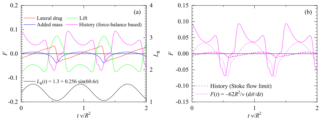
FIG. 10. Results for the various hydrodynamic forces on a bubble bouncing close to the wall. In panel (a), the left tick label corresponds to the force normalized by \pi R^2 \rho U^2/2 , while the right one corresponds to the wall distance L_R . In panel (b), different lines correspond to the estimated history force based on different methods. Results for the bubble trajectory were originally presented in the experiment of Ref. [3]. Details about the experimental condition: \nu = 1.08 \times 10^{-6} \text{m}^2/\text{s} , R = 0.385 \text{mm} , and \text{Re}_\infty = 130 .
