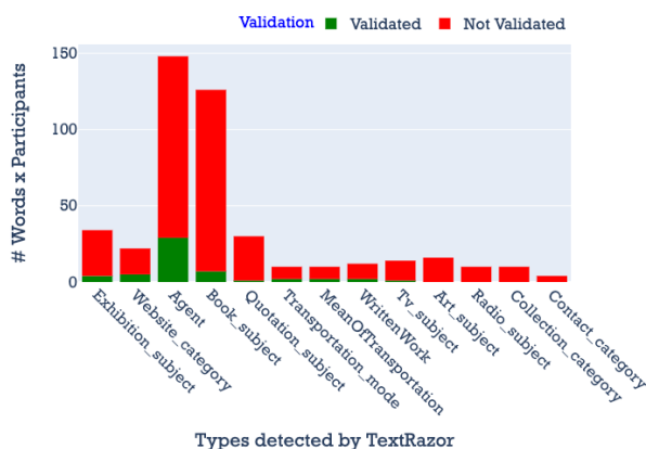
Fig. 8. Types misdetected by TextRazor
