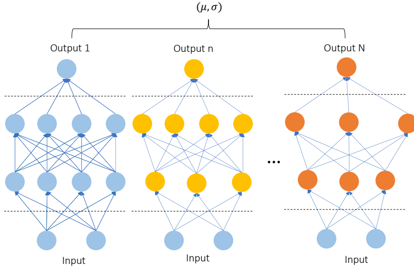
Figure 9: Example of an ensemble model with multiple neural networks. Parameter \mu is the mean or expectation of N distributions, \sigma is the standard deviation.
