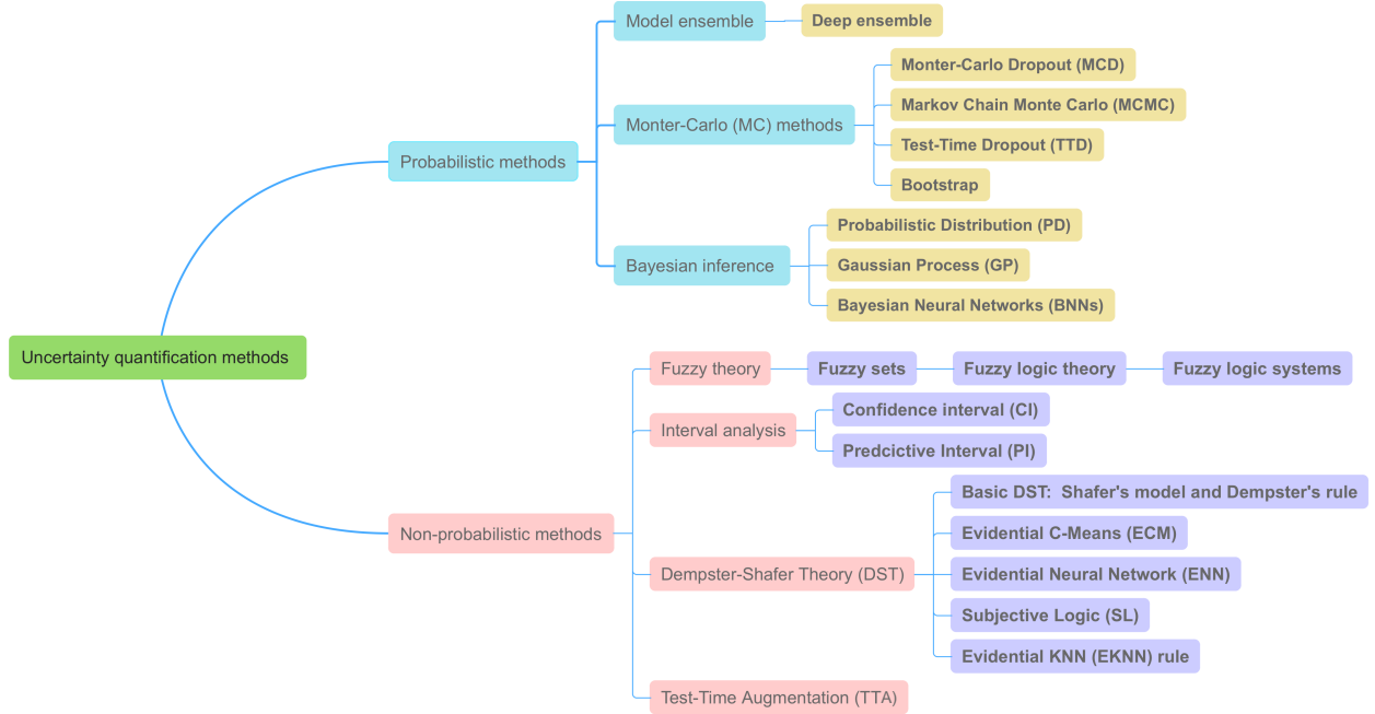
Figure 4: Overview of uncertainty quantification methods: Probabilistic and Non-probabilistic methods
