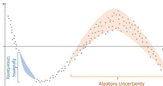
Figure 1: An example explanation of aleatory uncertainty inherently random and epistemic uncertainty caused by a lack of knowledge about the best analysis model (reproduced based on (Yang and Li, 2023))
