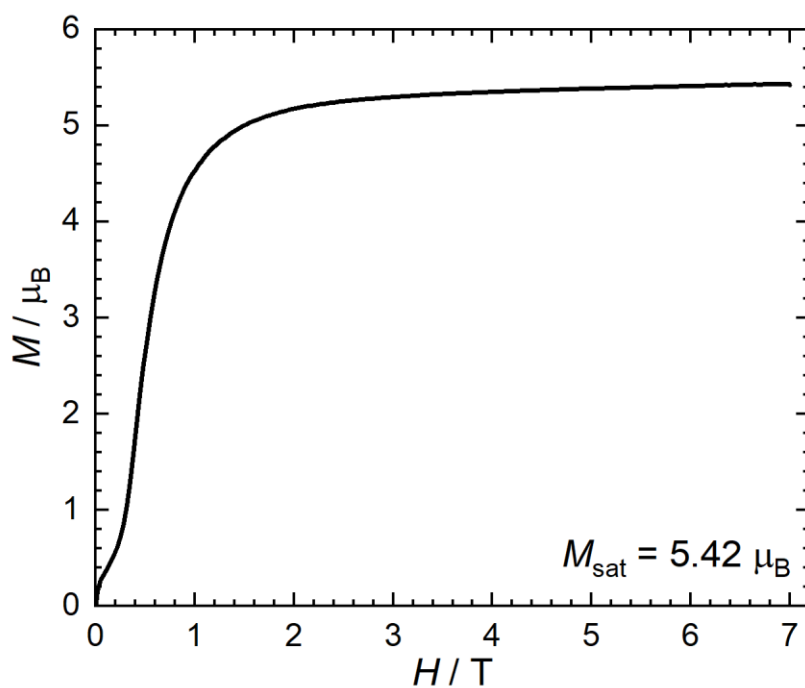
Figure S78. Field ( H ) dependence of the magnetization ( M ) (0–7 T) of 1-Dy suspended in eicosane at 2 K after cooling in zero field. Sweep rate is 22 \text{ Oe s}^{-1} ( 0.132 \text{ T min}^{-1} ).
