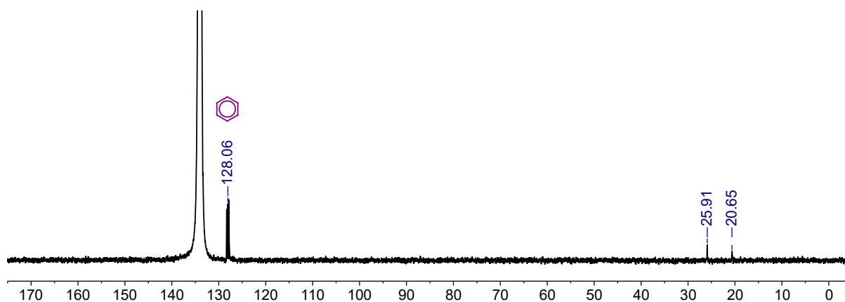
Figure S36. ^{13}\text{C}\{^1\text{H}\} DEPTQ NMR spectrum (100.60 MHz, \text{C}_6\text{D}_6 ) of 3-Dy at 298 K.
