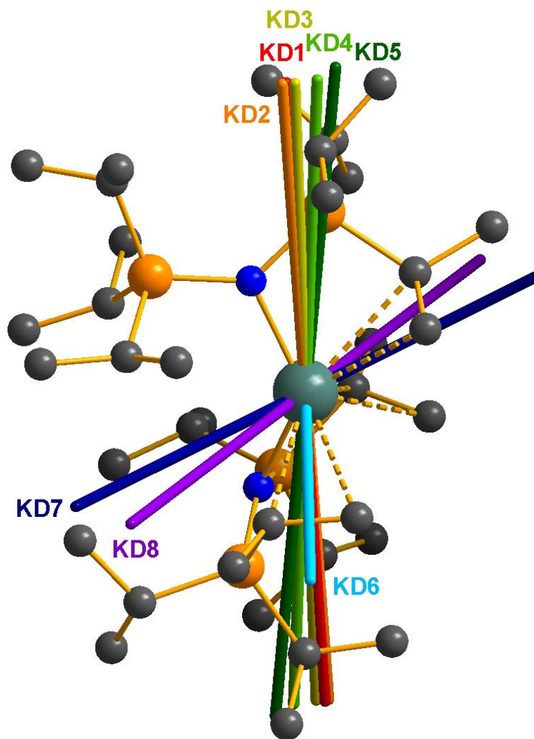
Figure S109. Structure of 1-Dy cation with overlaid g_z vectors for Kramer's doublets (KD1–KD8) calculated with CASSCF-SO. Hydrogen atoms are omitted for clarity.
