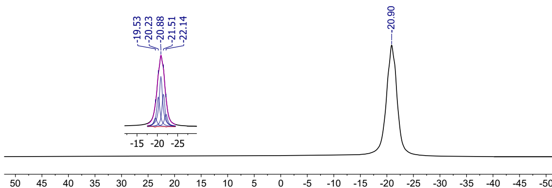
Figure S30. ^{11}\text{B} NMR spectrum (128 MHz, \text{C}_6\text{H}_4\text{F}_2 ) of 3-Y at 298 K. Inset: line fitting of the resonance as a broad pentet, using a generalized-Lorentzian form with no additional constraints, as implemented in MestReNova version 14.3.
