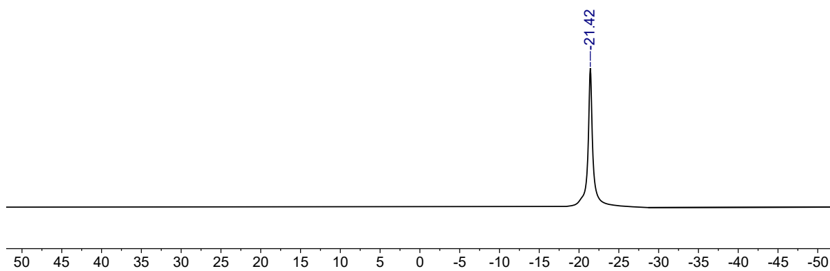
Figure S40. ^{11}\text{B}\{^1\text{H}\} NMR spectrum (128 MHz, \text{C}_6\text{D}_6 ) of 4-Y at 298 K.
