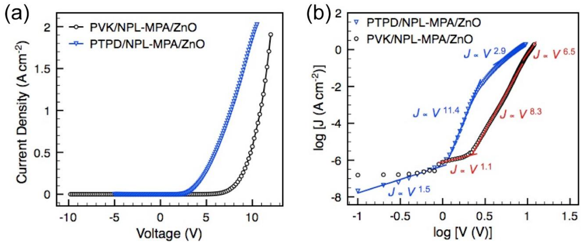
Figure 5. (a) Current-voltage characteristics showing both reverse and forward bias regimes indicating rectifying behaviour and (b) double logarithmic plot of the current-voltage characteristics of NPL-LEDs based employing PVK/NPL-MPA/ZnO (black circles) and PTPD/NPL-MPA/ZnO (blue triangles) as the active layers.
