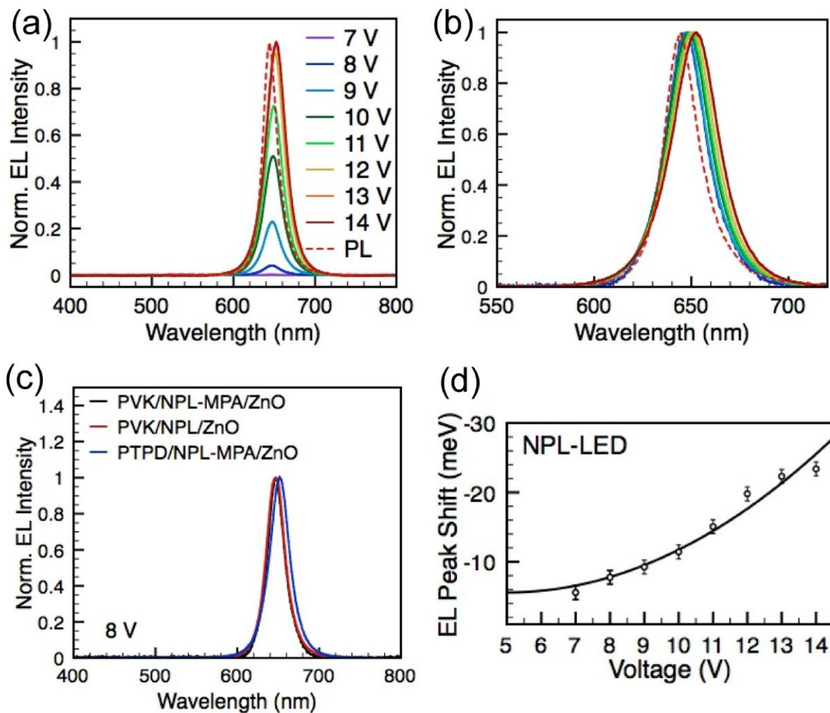
Figure 6. (a) Electroluminescence (EL) spectra of an optimized NPL-LED with the active layers based on the PVK/NPL-MPA/ZnO under different forward bias plotted together with the normalized PL spectra of the corresponding NPL films. The EL maximum associated with the highest applied voltage was normalized to 1. (b) The same EL spectra as (a) but with each
