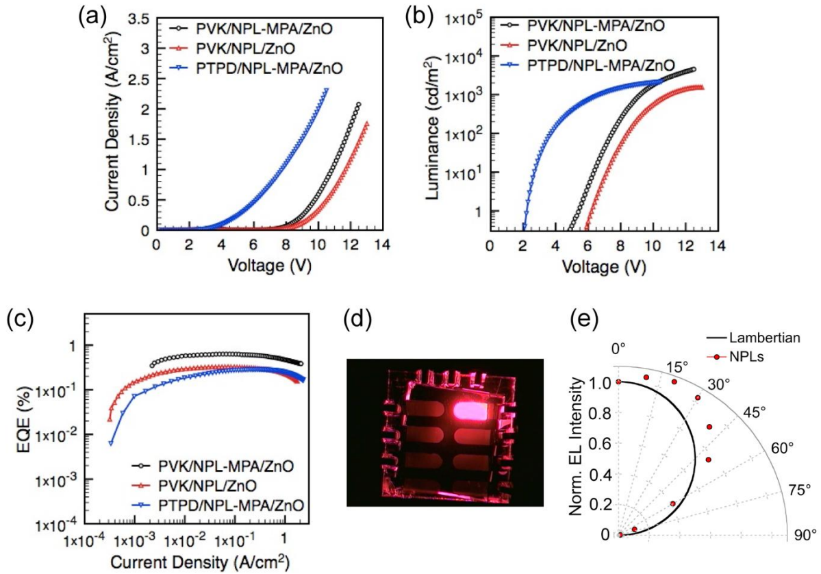
Figure 4. (a) Current density-voltage, (b) the corresponding luminance-voltage, and (c) EQE-current density characteristics of LEDs based on core/shell CdSe/CdZnS NPLs employing PVK/NPL-MPA/ZnO (black circles), PVK/NPL/ZnO (red triangles) and PTPD/NPL-MPA/ZnO (blue triangles) layers, sandwiched between ITO/PEDOT:PSS and Al. NPL-MPA refers to NPLs with ligands exchanged to MPA. (d) Photograph of a typical NPL-LED (with an emitting area of 4 \text{ mm}^2 ) under an applied voltage of 10 V. (e) Normalized angular emission profiles of a representative NPL-LED measured on a rotation stage (with device edges masked). The dark line represents the Lambertian emission profile.
