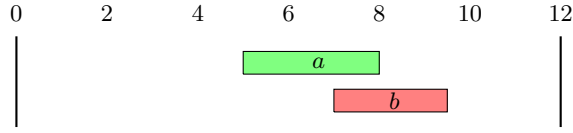
Fig. 9. Tipomset of accepting path in HDTA of Ex. 27
