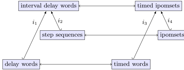
Fig. 6. Different types of language semantics: below, for languages of timed automata; middle, for languages of HDAs; top, for languages of HDTAs. Vertical arrows denote injections, horizontal arrows bijections.
