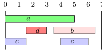
Fig. 8. Gluing T_1 * T_2 , see Ex. 17
