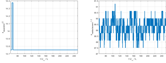
Figure 7: History of the mean location in the spanwise direction of the abscissa along the flat plate of the separation point, on the left, and the reattachment point, on the right.
