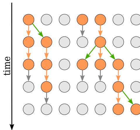
Figure 2: Directed percolation on an array of 7 sites. Each row represents a different time step, green arrows indicate birth, gray arrows death, and orange arrows survival.
