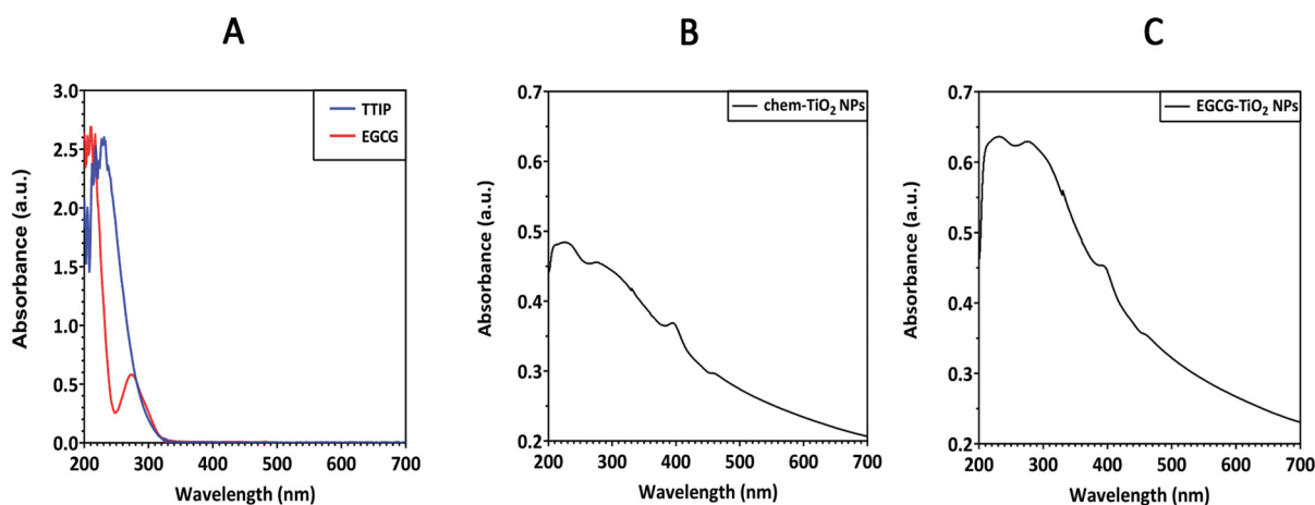
Figure 1. UV-VIS absorbance spectra of (A) TTIP and EGCG precursors, (B) chem-TiO 2 NPs and (C) EGCG-TiO 2 NPs.
