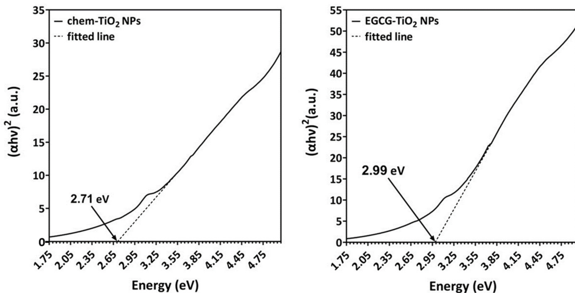
Figure 2. Tauc plot of chem-TiO 2 NPs (left) and EGCG-TiO 2 NPs (right). Arrows indicate the value of the bandgap energy estimated by linear fit.
