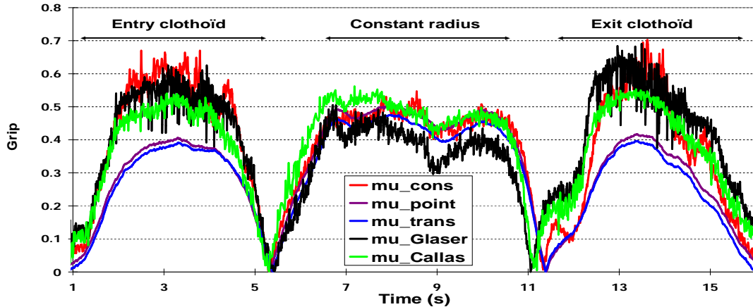
Figure 6. Consumed grip, v=82\text{km/h} , r=110\text{m} , wet surface
