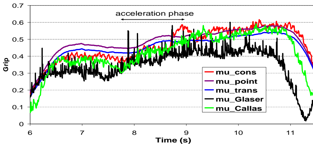
Figure 7. Consumed grip, v=80\text{km/h} , r=110\text{m} , dry surface, acceleration
