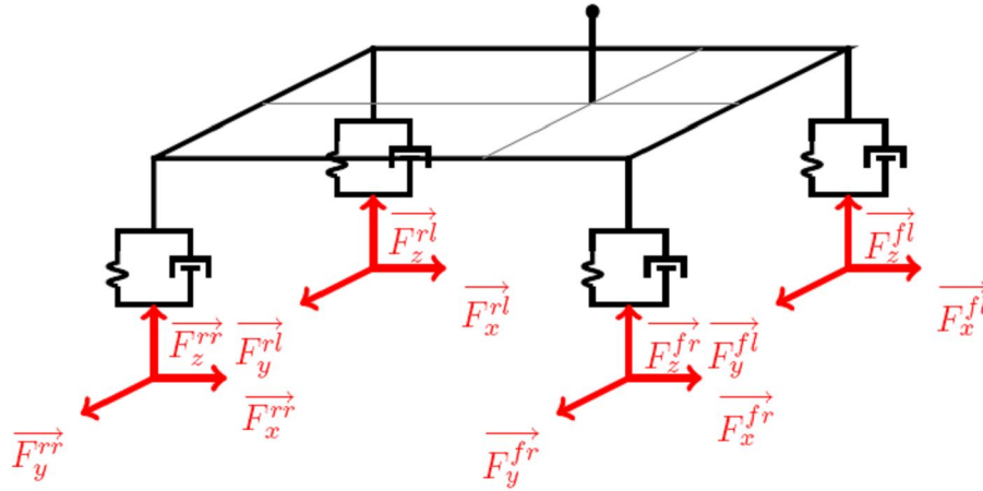
Figure 3. Four wheels model
