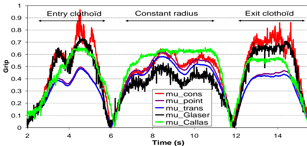
Figure 5. Consumed grip, v=88\text{km/h} , r=110\text{m} , dry surface
