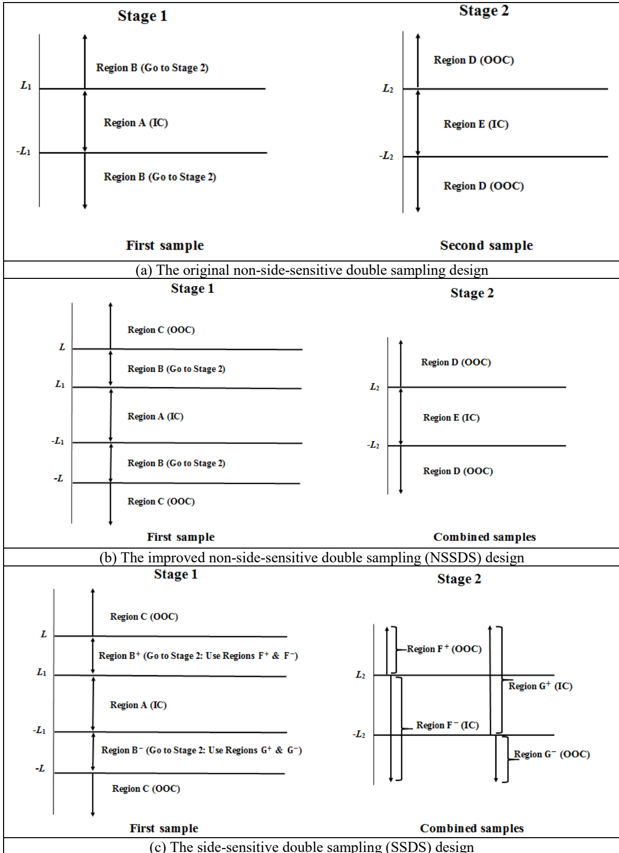
Figure 1: The charting regions in stages 1 and 2 of the different double sampling designs
