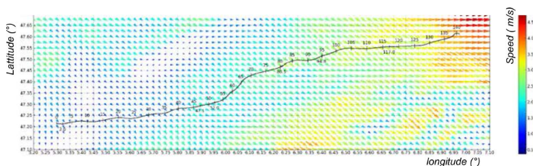
Figure 1 Example of the discretized wind field computed with the AROME model, around the 140 km high-speed line
