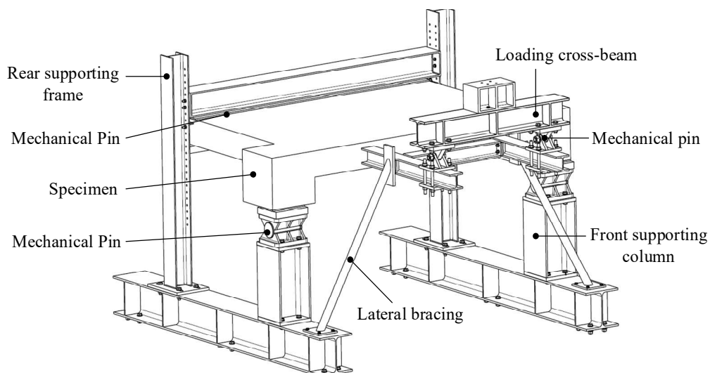
Figure 4: Test setup.
