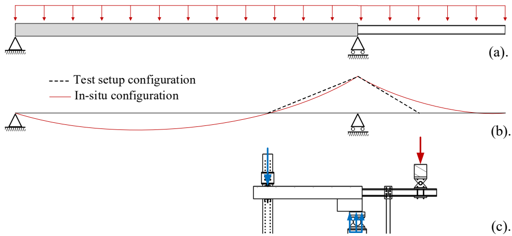
Figure 3: Specimen design: (a). Configuration of real loads on floor-to-balcony connection. (b). bending moment diagrams. (C). Configuration of testing.
