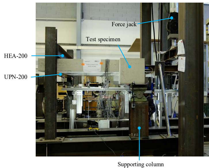
Figure 6: Actual photo of the test setup.
