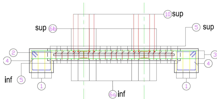
Figure A3: Cut 1-1.
