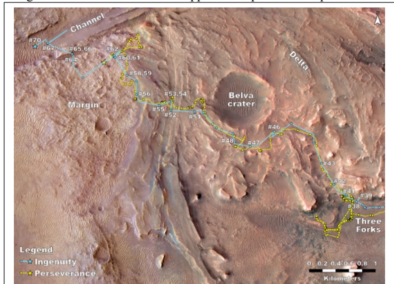
Fig. 1. Color HiRISE image showing ground and flight traverses of Mars 2020 rover and the helicopter in Jezero crater. Main terrains and landing sites after selected flights shown in white. Flight 66 is where the helicopter spent conjunction and conducted the aeolian change experiment.
