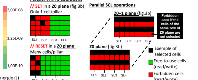
Fig. 22: Illustration of parallel write and SCL operations of our 3D RRAM architecture. Each word can be addressed in a row of the cube. The parallel SCL operation is performed on the same row of the different 'Z' planes of the 3D RRAM cube.
