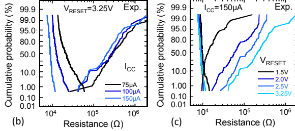
Fig. 13: (a) Schematics of our 4kbits 1T1R memory array integrating TiN/HfO 2 /5nm/Ti 5nm/TiN OxRAMs. LRS and HRS distributions of OxRAM memory cells for (b) different I_{CC} and (c) V_{RESET} . High values of I_{CC} and V_{RESET} are preferable to ensure a large memory window (MW) between HRS and LRS states.
