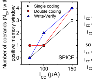
Fig. 20: Max. number of operands ( N_{OP} ) with positive MW enabling scouting logic (SPICE simulation).
