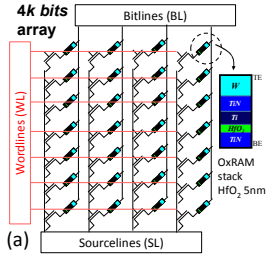
Fig. 13: (a) Schematics of our 4kbits 1T1R memory array integrating TiN/HfO 2 /5nm/Ti 5nm/TiN OxRAMs. LRS and HRS distributions of OxRAM memory cells for (b) different I_{CC} and (c) V_{RESET} . High values of I_{CC} and V_{RESET} are preferable to ensure a large memory window (MW) between HRS and LRS states.
