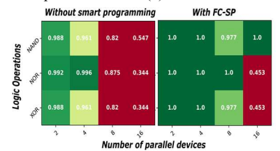
Fig. 12: Experimental success rate for NAND, NOR and XOR scouting logic operations without smart programming and with FC-SP. FC-SP renders IMC possible with up to 16 parallel operands.
