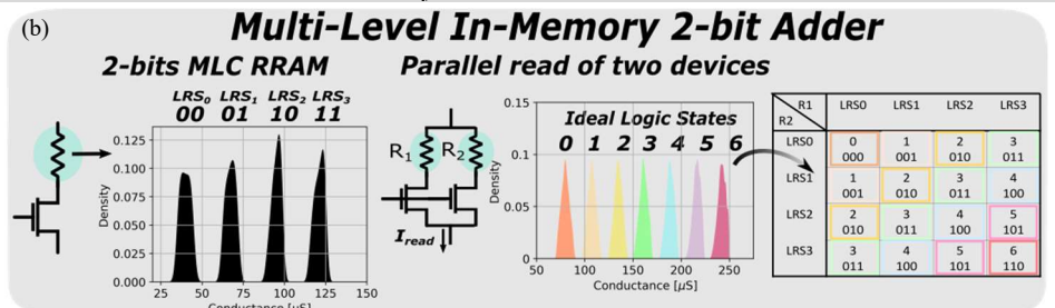
Fig. 9: Conventional architecture needed for a 2-bit adder (a) and proposed Multi-Level In-Memory 2-bit adder based on two parallel RRAMs (b).
