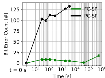
Fig. 7: Bit Error Count on time for the most error prone level (level 0 in Fig. 4) one month) for the 3 FC-SP and PC-SP.
