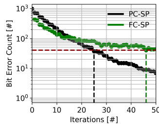
Fig. 6: Bit Error Count (BEC) as a function of the number of iterations during PC-SP and FC-SP.
