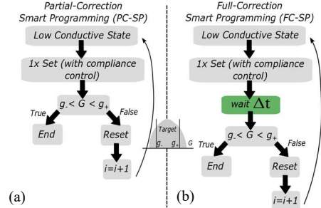
Fig. 2: MLC Programming strategies flow: Partial Correction Smart Programming (PC-SP) [8] (a) and with Full Correction Smart Programming (FC-SP) (b).
