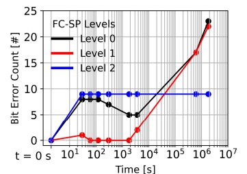
Fig. 8: Bit Error Count on time (up to one month) for the 3 FC-SP programmed levels.
