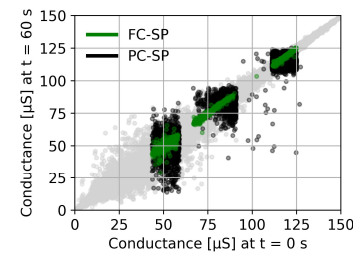
Fig. 5: Relaxation effect for FC-SP and PC-SP after 60 seconds. Grey color represents distributions without smart programming.
