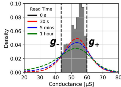
Fig. 3: Conductance distribution programmed with FC-SP strategy and the High Resistive State (HRS) just after programming (black) and after 1 hour (green).
