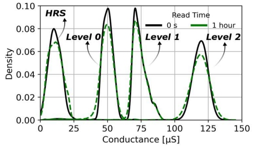
Fig. 4: Three conductance levels programmed with FC-SP strategy and the High Resistive State (HRS) just after programming (black) and after 1 hour (green).
