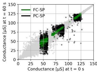
Fig. 5: Relaxation effect for FC-SP and PC-SP after 60 seconds. Grey color represents distributions without smart programming.
