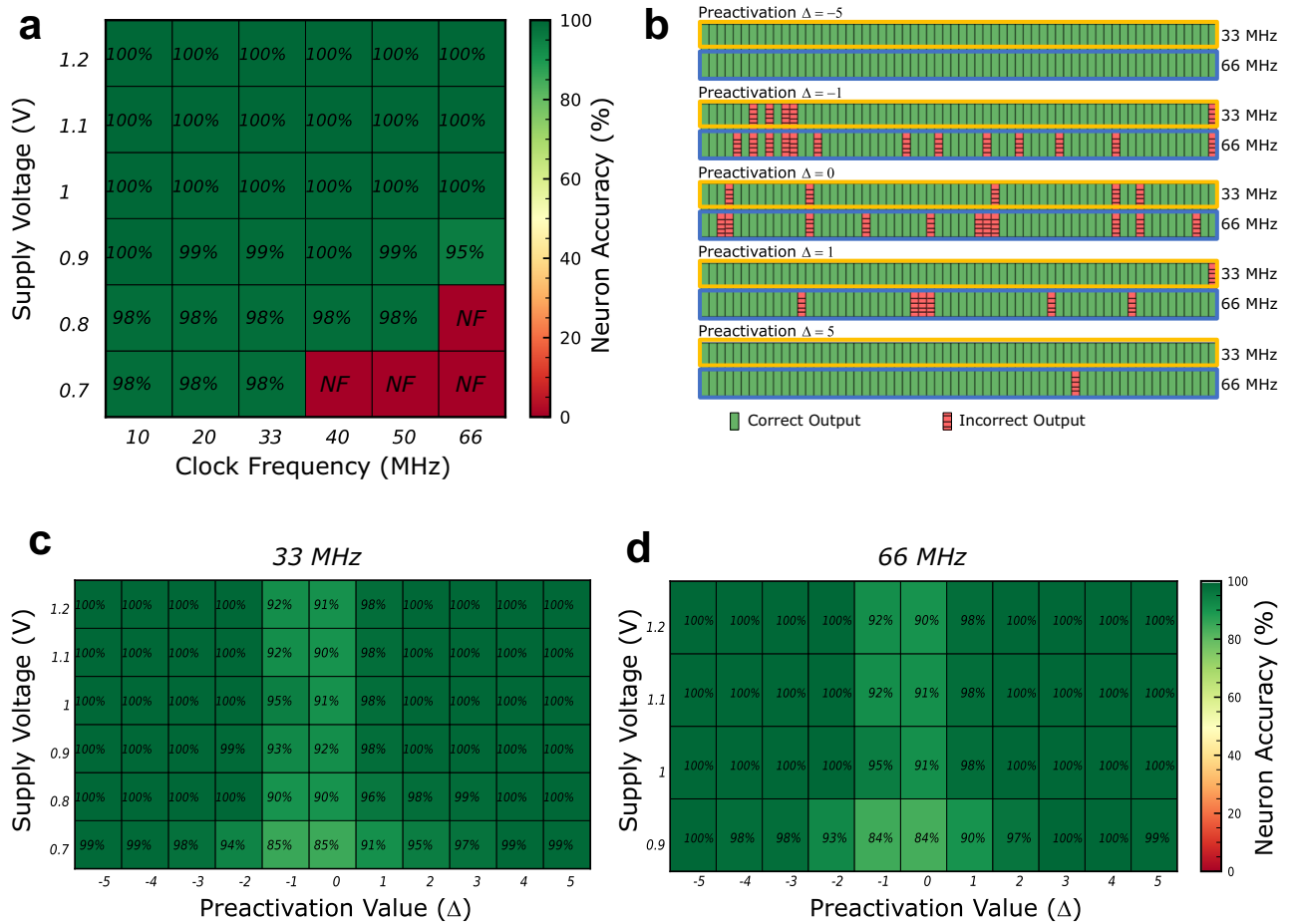
Fig. 3 | Accuracy of the memristor-based binarized neural network. a Measured schmoo plot, presenting mean accuracy of the output neuron activations, for different operation frequency and supply voltage. They were obtained using patterns of weights and inputs chosen to cover all possible neuron preactivations (see Methods). NF means non-functional. b Measurements of 64 neurons with
