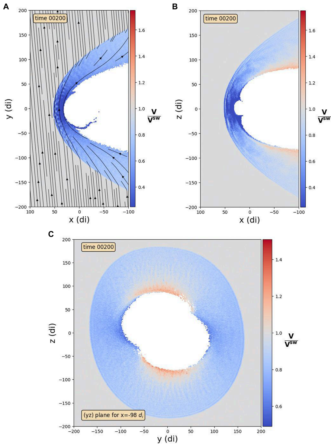
FIGURE 2 Colormap of the velocity in the magnetosheath in different planes. The velocity is represented as a ratio between the local velocity and the velocity in the solar wind ( V^{sw} = 400 km/s). The regions where the velocity is equal to the velocity in the solar wind are shown in grey. Velocities slower or faster than V^{sw} are shown respectively in blue or red. The magnetosphere (simply defined here as where the density is below 4 particles per \text{cm}^3 ) is shown in white. The panels represent the velocity of the plasma in, respectively; (A) the (Oxy) plane, (B) the (Oxz) plane, and (C) the plane (yz) for x = -98 d_i . The magnetic field lines are represented in the (Oxy) plane only (A) , because the interplanetary magnetic field has no z component.
