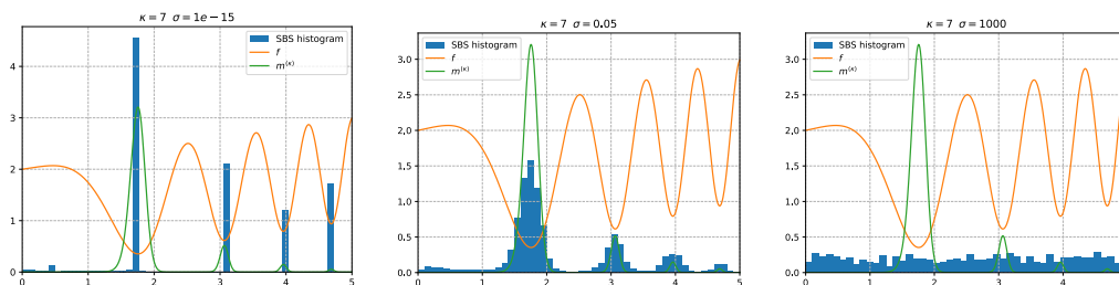
Figure 3. Illustration of the exploration/exploitation trade-off in SBS with different values of \sigma . In blue, the repartition of the particles, in orange, x \mapsto \cos(x^2) + x/5 + 1 , in green m^{(\kappa)} .
