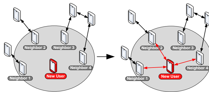
Figure 8. Creating links with Gnc and Gc group members.
