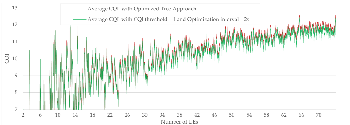
Figure 22. Comparison of the average CQI between the optimized tree approach and the customized approach (CQI threshold = 1 and optimized interval = 2 s).
