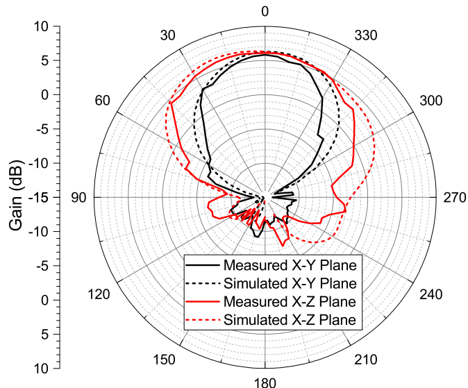
Fig. 10. Measured and simulated radiation pattern of the antenna at 26 GHz, on X-Y plane ( \theta = 90 deg) and X-Z plane ( \phi = 0 ).
