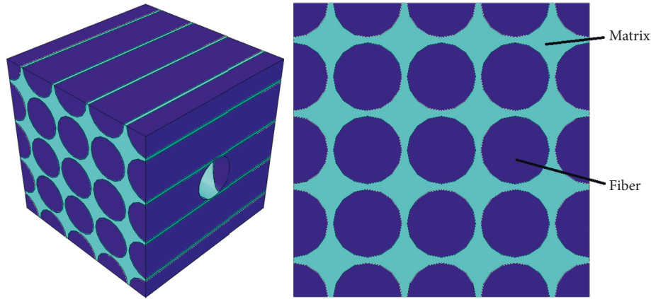
FIGURE 9: Composite micromechanical model.
