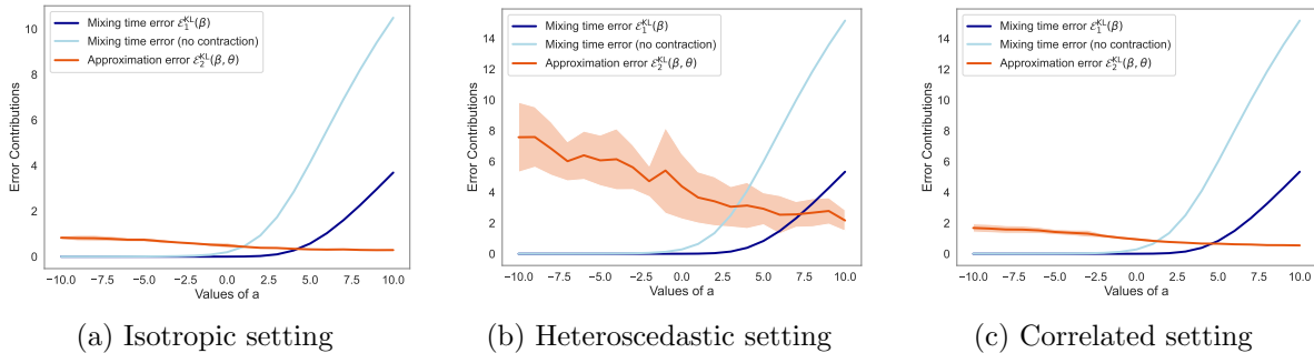
Figure 12: Error terms contribution from Theorem 3.1 displayed from the same examples as in Figure 2 (top).
