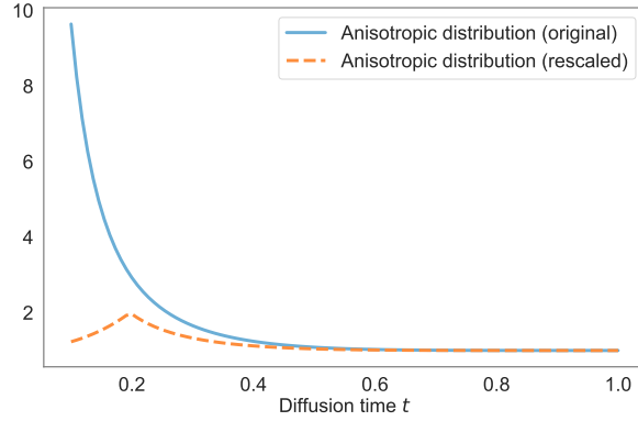
Figure 16: Comparison of the ratio strong concavity / Lipschitz continuity for the true score function \nabla \log p_t in the Heteroscedastic setting before rescaling (Figure 14 (b)) and after rescaling (Figure 15 (d)) throughout diffusion time t \in (0, T] .
