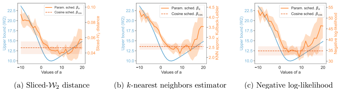
Figure 18: Upper bound and empirical distances between the data distribution and the generated samples for different metrics on a mixture of 25 Gaussian variables dataset in dimension 50.
