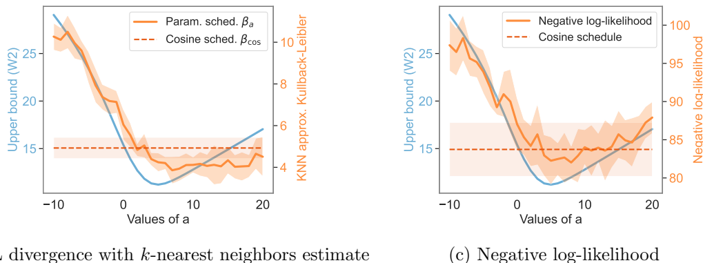
Figure 17: Upper bound and empirical distances between the data distribution and the generated samples for different metrics on a Funnel dataset in dimension 50.
