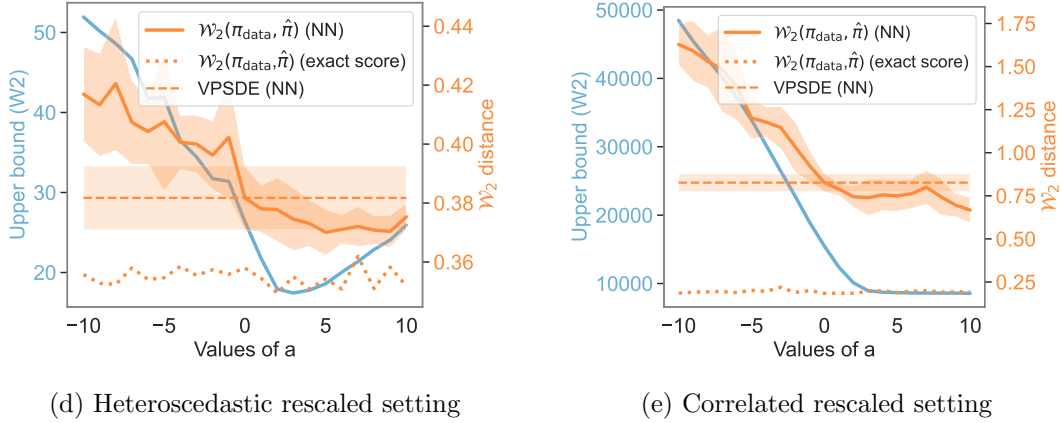
Figure 15: Comparison of the empirical 2-Wasserstein distance on rescaled datasets for (d) \pi_{\text{scale}}^{(\text{heterosc})} , (e) \pi_{\text{scale}}^{(\text{corr})} .
