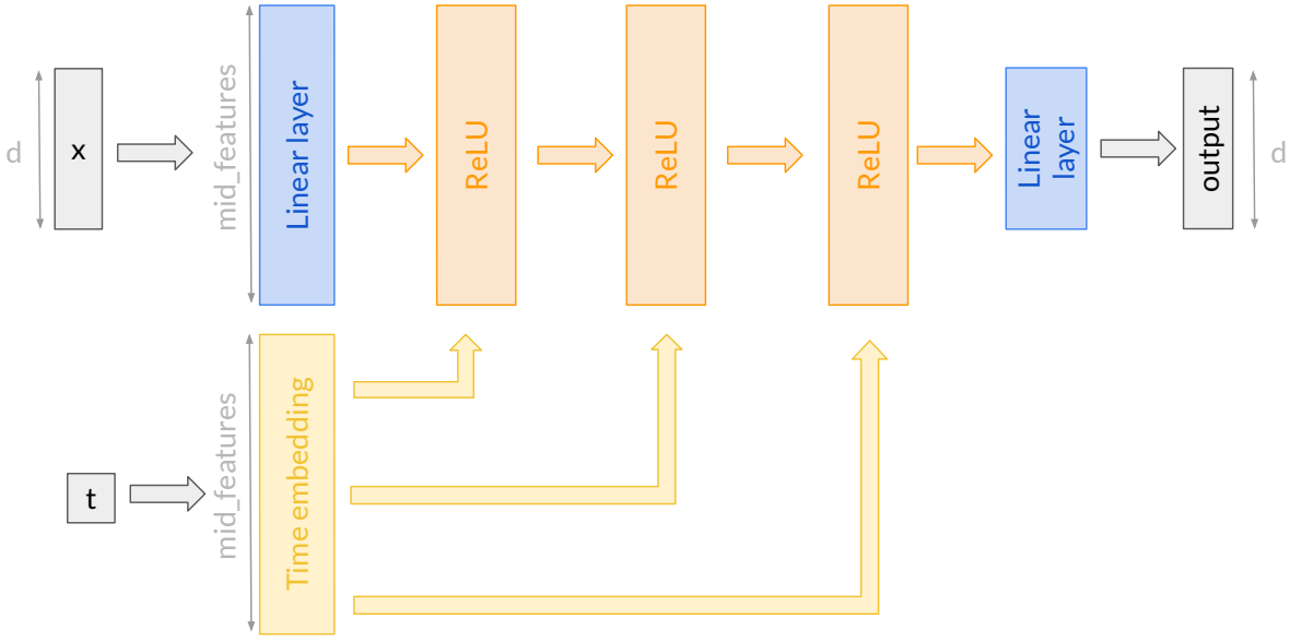
Figure 11: Neural network architecture. The input layer is composed of a vector x in dimension d and the time t . Both are respectively embedded using a linear transformation or a sine/cosine transformation (Nichol and Dhariwal, 2021) of width mid_features . Then, 3 dense layers of constant width mid_features followed by ReLU activations and skip connections regarding the time embedding. The output layer is linear resulting in a vector of dimension d .
