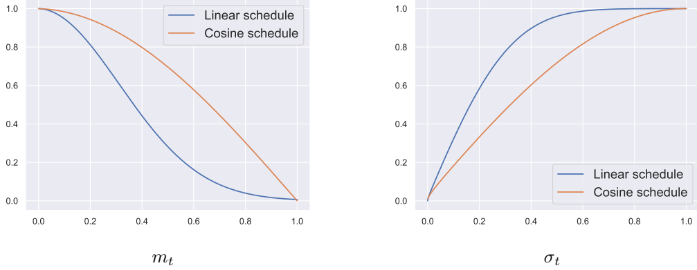
Figure 9: Evolution of m_t and \sigma_t for both the cosine schedule (orange) and the linear schedule (blue) w.r.t. time, with s = 0.021122 and \sigma^2 = 1 . We clip the value of \beta_{\text{cos}} by 200 for better visualization.
