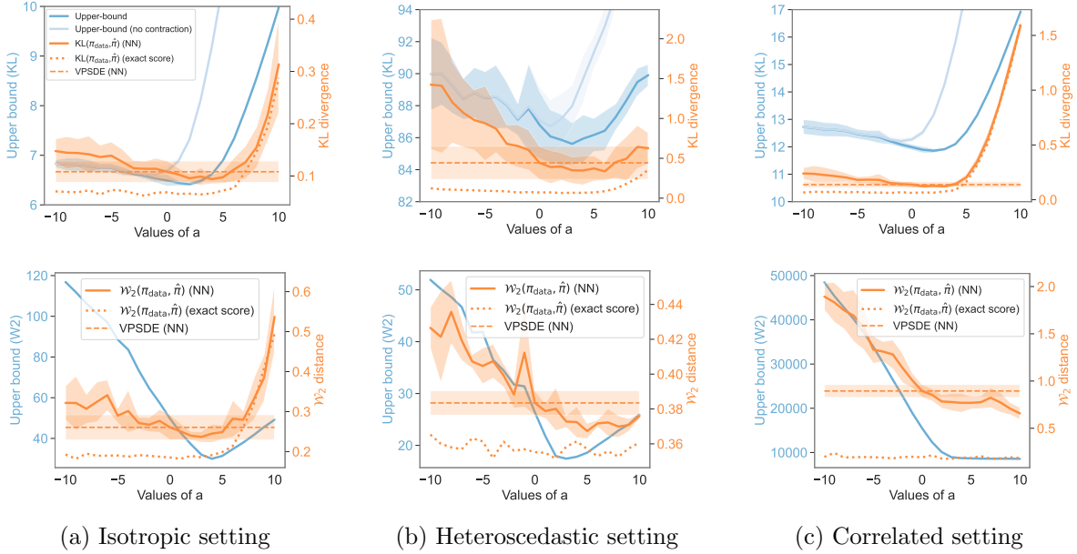
Figure 10: Comparison of the empirical KL divergence (mean \pm std over 30 runs) (top) and \mathcal{W}_2 distance (mean \pm std over 10 runs) (bottom) between \pi_{\text{data}} and \hat{\pi}_N^{(\beta, \theta)} (orange) and the related upper bounds (blue) from Theorem 3.1 and Theorem 4.2 across parameter a for noise schedule \beta_a , d = 50 with Exponential Integrator discretization scheme. We also show the metrics for the linear VPSDE model (dashed line) and our model (dotted line) with exact score evaluation.
