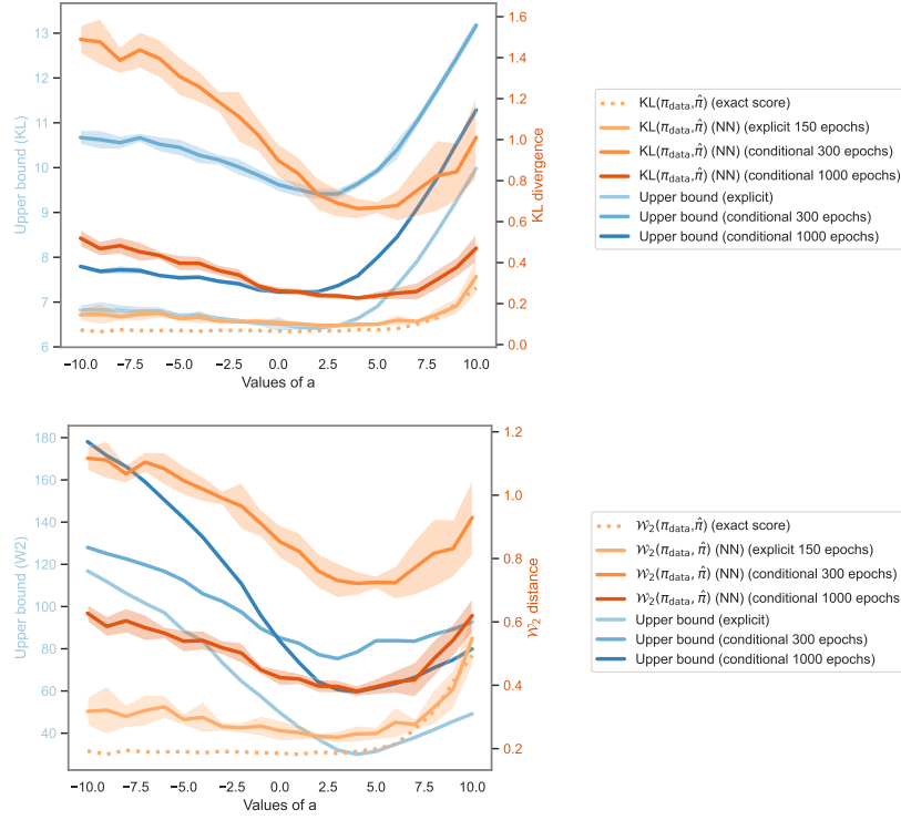
Figure 21: Comparison of the empirical KL divergence (top) and the \mathcal{W}_2 distance (bottom) (mean value \pm std over 10 runs) between \pi_{\text{data}} = \pi_{\text{data}}^{(\text{iso})} and \hat{\pi}_N^{(\beta_a, \theta)} (in orange) and the upper bound of Theorem 3.1 (top) and of Theorem 4.2 (bottom) (in blue) w.r.t. the parameter a used in the definition of the noise schedule \beta_a , for d = 50 .
