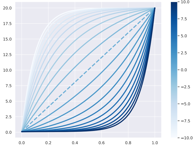
Figure 6: Evolution of noise schedules \beta_a w.r.t. time, for different values of parameter between -10 to 10 . The linear case a = 0 (Song and Ermon, 2019; Song et al., 2021) is dashed.
