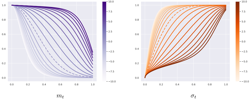
Figure 7: Evolution of m_t and \sigma_t over time, for different choices of a in the noise schedule \beta_a used in see Section 5. The stationary distribution of the forward process \sigma^2 is set to 1. The range for a spans from -10 to 10, with the dashed line representing the linear schedule as proposed originally in the VPSDE models (Song et al., 2021).
