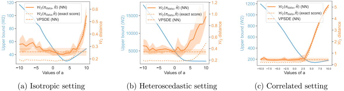
Figure 14: Comparison of the empirical 2-Wasserstein distance (mean value \pm std over 10 runs) between \pi_{\text{data}} and \hat{\pi}_N^{(\beta_a, \theta)} (in orange) and the upper bound from Theorem 4.2 (in blue) w.r.t. the parameter a used in the definition of the noise schedule \beta_a , for d = 50 . We also represent the 2-Wasserstein distances obtained with the linear VPSDE model (dashed line) and the one obtained with the parametric model (dotted line) when the score is not approximated but exactly evaluated. The data distribution \pi_{\text{data}} is chosen Gaussian, corresponding to (a) \pi_{\text{data}}^{(\text{iso})} , (b) \pi_{\text{data}}^{(\text{heterosc})} and (c) \pi_{\text{data}}^{(\text{corr})} .
