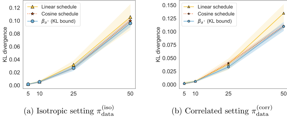
Figure 13: Comparison of the empirical KL divergence (mean value \pm std over 10 runs) between \pi_{\text{data}} and the generative distribution \hat{\pi} for different values of the dimension. The generative distributions considered are \hat{\pi}_N^{(\beta_{a^*}, \theta)} obtained by the time-inhomogeneous SGM for \beta_{a^*} (blue plain), \hat{\pi}_N^{(\beta_0, \theta)} obtained by a standard linear VPSDE model (yellow dashed) and \hat{\pi}_N^{(\beta_{\text{cos}}, \theta)} obtained by using a cosine schedule (orange dotted).
