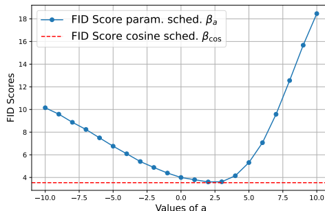
Figure 5: FID Scores using 50,000 generated samples for the parametric and cosine schedules (CIFAR-10 dataset).
