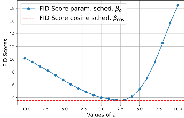
Figure 19: FID scores on 50 000 generated samples using pre-trained models from Karras et al. (2022) with different noise schedules from the parametric family (9) and cosine schedule.
