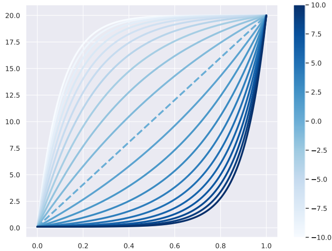
Figure 1: Evolution of noise schedules \beta_a w.r.t. time, for different values of parameter between -10 to 10 . The original choice of noise schedule in the VPSDE case (Ho et al., 2020) is shown as a dashed line, corresponding to a linear noising function.
