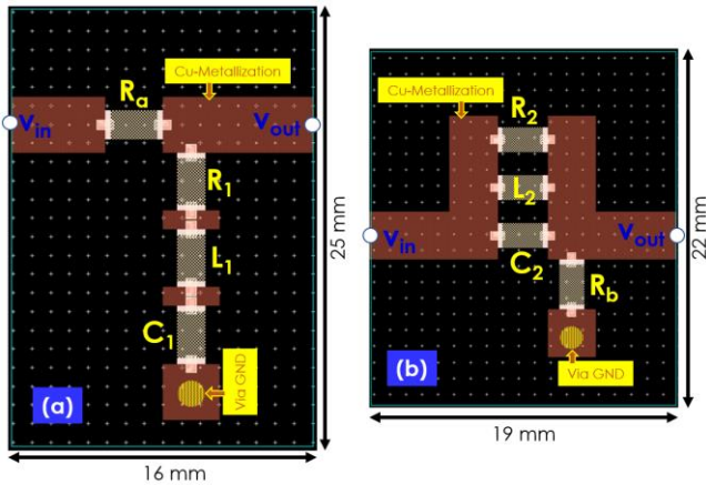
FIGURE 3. Momentum® layouts of designed (a) RLC-series and (b) RLC-parallel PoC circuits.
