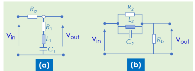
FIGURE 1. (a) RLC-series and (b) RLC-parallel network-based BP-NGD topologies.
