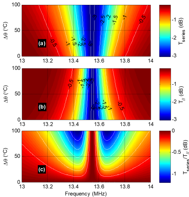
FIGURE 5. Thermo-frequency variable mappings of (a) RLC-series, (b) RLC-parallel VTF magnitudes and (c) ratio of both magnitudes from the circuits shown in Figs. 2.
