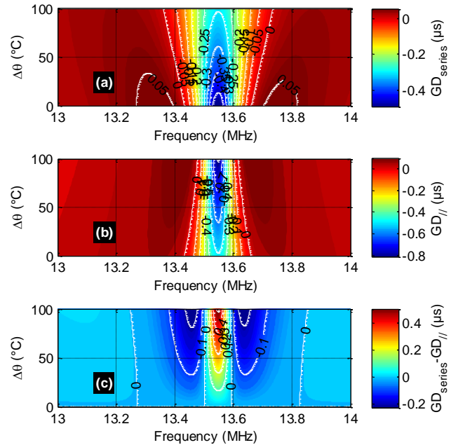
FIGURE 6. Thermo-frequency variable mappings of (a) RLC-series, (b) RLC-parallel VTF GDs and (c) their algebraic difference from the circuits shown in Figs. 2.
