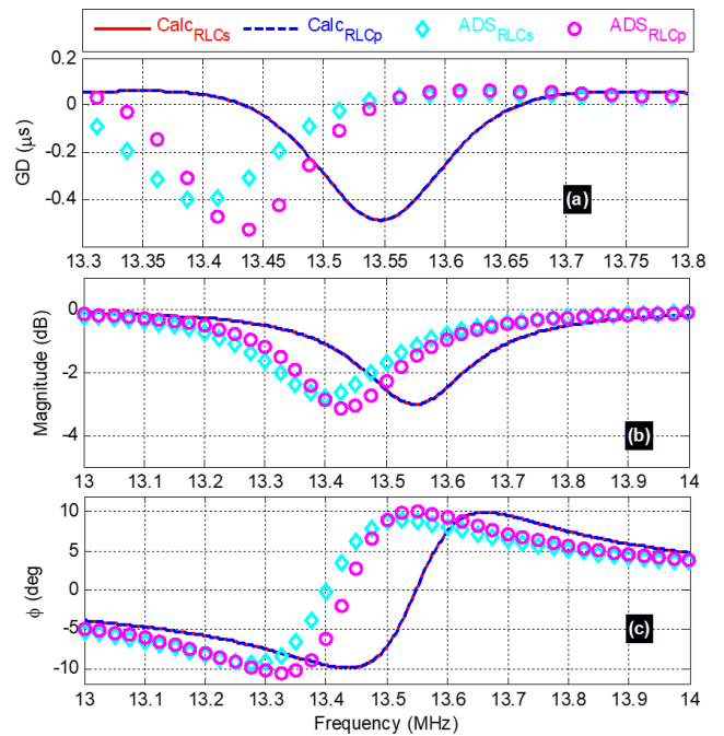
FIGURE 4. Comparisons of calculated and simulated VTFs: (a) GD, (b) magnitude and (c) phase from the RLC-series and RLC-parallel circuits shown in Figs. 2 and Figs. 3.
