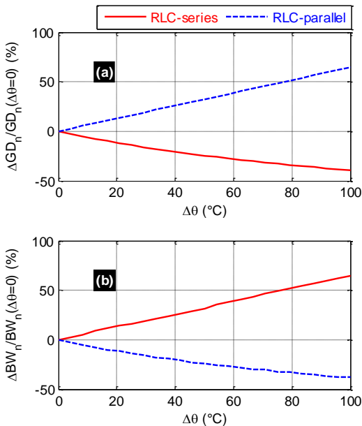
FIGURE 8. Relative variations of (a) NGD value and (b) NGD BW versus temperature variation.
