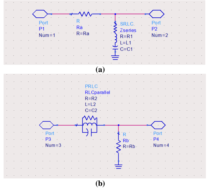
FIGURE 2. ADS® schematic of designed (a) RLC-series and (b) RLC-parallel circuits.
