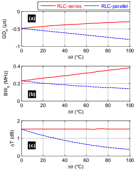
FIGURE 7. Variation of (a) NGD value and (b) NGD BW of circuits shown in Figs. 5 versus temperature variation.
