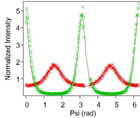
Figure 2: Normalized scattering intensity as a function of angle \psi for a 30 g/L 6-Cl gel and 0.15% BId-T3-Na under a shear of 3000 \text{ s}^{-1} . In red: scattering intensity obtained in the radial position. In green: scattering intensity obtained in the tangential position. Crosses represent the experimental points and solid lines represent the fit of the experimental data with Equation 2.
