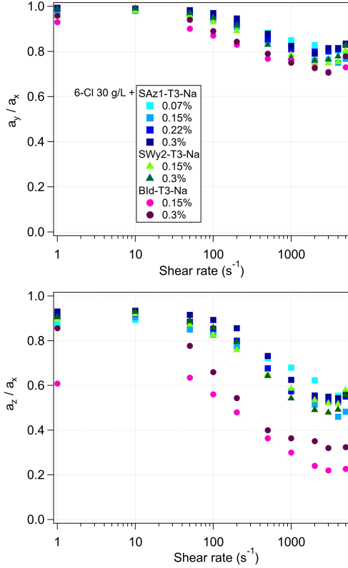
Figure 6: Evolution of the anisotropic parameters ratios a_y/a_x and a_z/a_x as a function of shear rate for 6-Cl gels at 30 g/L for different clay volume fractions. The same legend is used for both figures.
