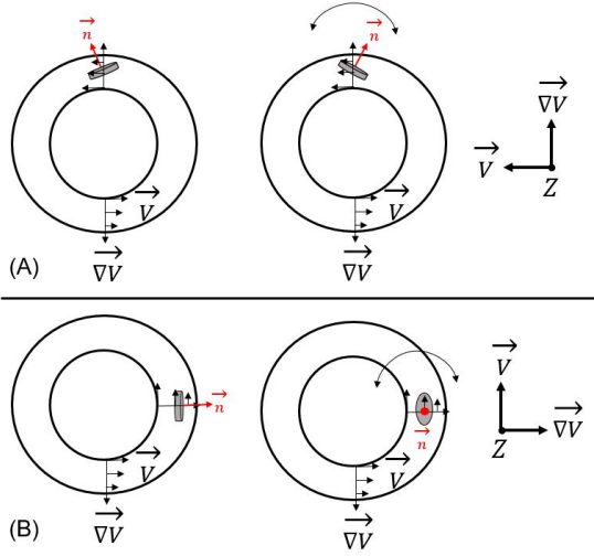
Figure 3: (A) Rotation of the normal vector \vec{n} in the plane (\vec{\nabla V}, \vec{V}) around the axis Z as described by the ratio of anisotropic parameters a_z/a_x . (B) Rotation of the normal vector \vec{n} in the plane (\vec{\nabla V}, Z) around the axis represented by \vec{V} as described by the ratio of anisotropic parameters a_y/a_x .
