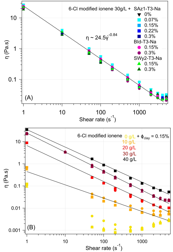
Figure 4: (A) Evolution of viscosity versus shear rate for 30 g/L 6-Cl gels for different clay volume fractions. The black solid line represents the power law fit of the experimental data for the 30 g/L 6-Cl gel and 0.15% SAz1-T3-Na. (B) Evolution of viscosity as a function of shear rate for gels with different concentrations of 6-Cl for a volume fraction of 0.15% clay and for the corresponding 0.15% clay suspensions. Bid-T3-Na is represented by circles, SAz1-T3-Na by squares and SWy2-T3-Na by triangles. The black solid lines represent the power law fits of the experimental data.
