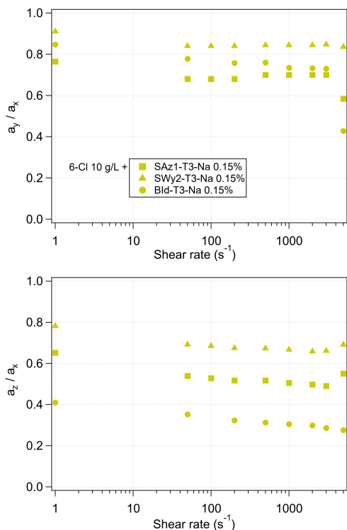
Figure 8: Evolution of the anisotropic parameters ratios a_y/a_x and a_z/a_x as a function of shear rate for 6-Cl gels at 10g/L and for 0.15% of clay volume fraction. The same legend is used for both figures.
