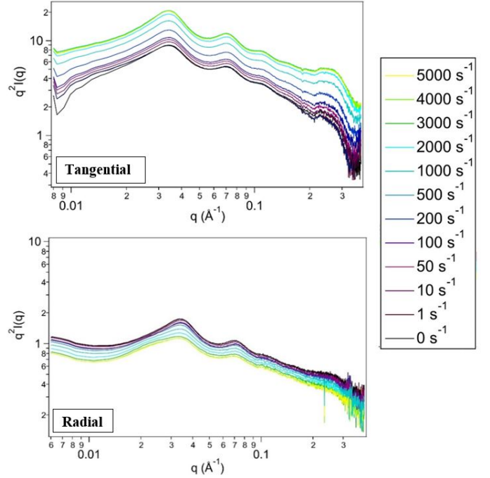
Figure 5: Evolution of the structure factor q^2 I(q) as a function of the scattering vector q for 6-Cl gel at 30 g/L and 0.15% of SAz1-T3-Na at different shear rates in the tangential and radial positions.
