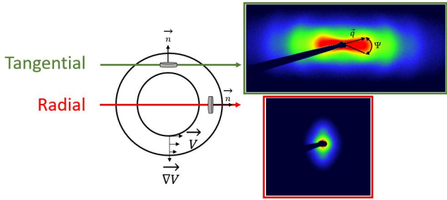
Figure 1: Cross-section of the Couette geometry. 2D SAXS images obtained, under a shear of 3000 \text{ s}^{-1} , in the tangential position (green) and in the radial position (red) for 30 g/L 6-Cl gel and 0.15% BId-T3-Na. The vectors represent the velocity lines and the velocity gradient. The angle \psi representing the orientation of the scattering vector in the plane of the detector is shown in the scattering image in the tangential position.
