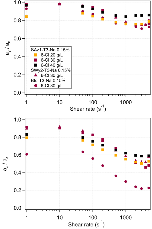
Figure 7: Evolution of the anisotropic parameters ratios a_y/a_x and a_z/a_x as a function of shear rate for 6-Cl gels at different concentration and with a clay volume fraction fixed at 0.15%. The same legend is used for both figures.
