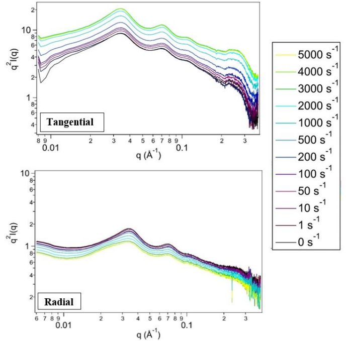
Figure 5: Evolution of the structure factor q^2 I(q) as a function of the scattering vector q for 6-Cl gel at 30 g/L and 0.15% of SAz1-T3-Na at different shear rates in the tangential and radial positions.
